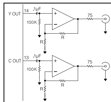
Fig. 7 - Video Output
