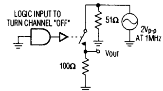
Figure 3. Off-Isolation Rejection Ratio
