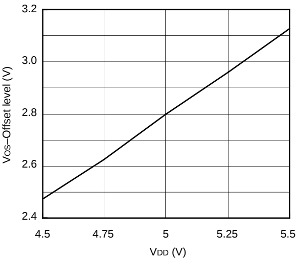
Offset level vs. V_{\text{DD}} (Typ.)
