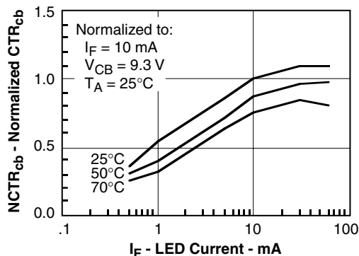
Figure 8. Normalized CTR_{cb} versus LED current and temperature
