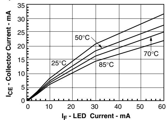
Figure 6. Collector-emitter current versus temperature and LED current
