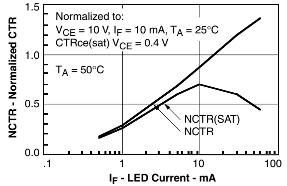
Figure 3. Normalized non-saturated and saturated CTR at T_A = 50^\circ\text{C} versus LED current
