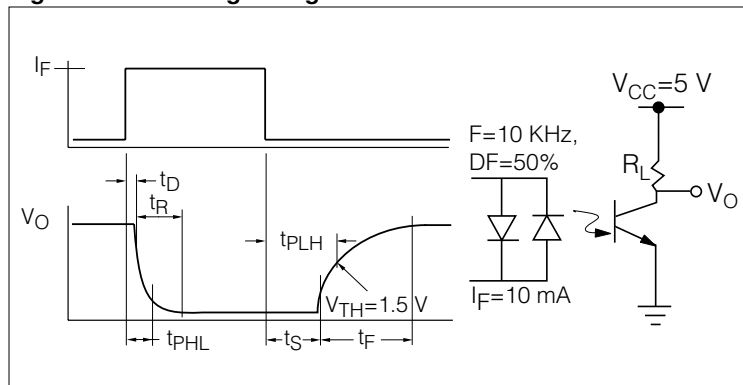
Figure 14. Switching timing and schematic
