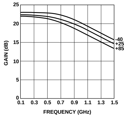
Figure 4. Gain vs. Frequency and Temperature.
