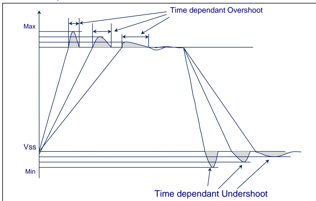
Figure 18. Maximum Acceptable Overshoot/Undershoot Waveform
