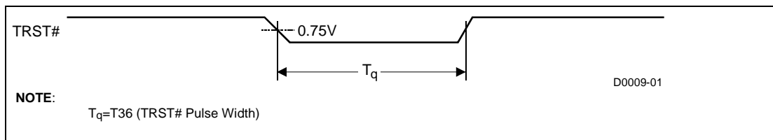
Figure 14. Test Reset Timings
