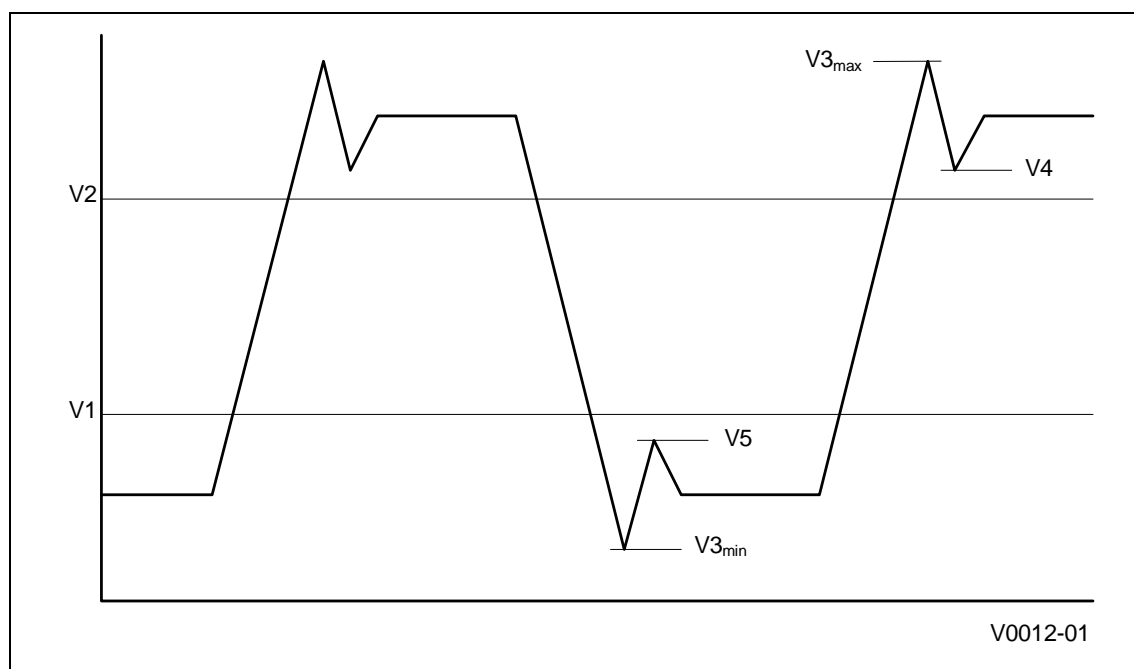
Figure 17. BCLK/PICCLK Generic Clock Waveform
