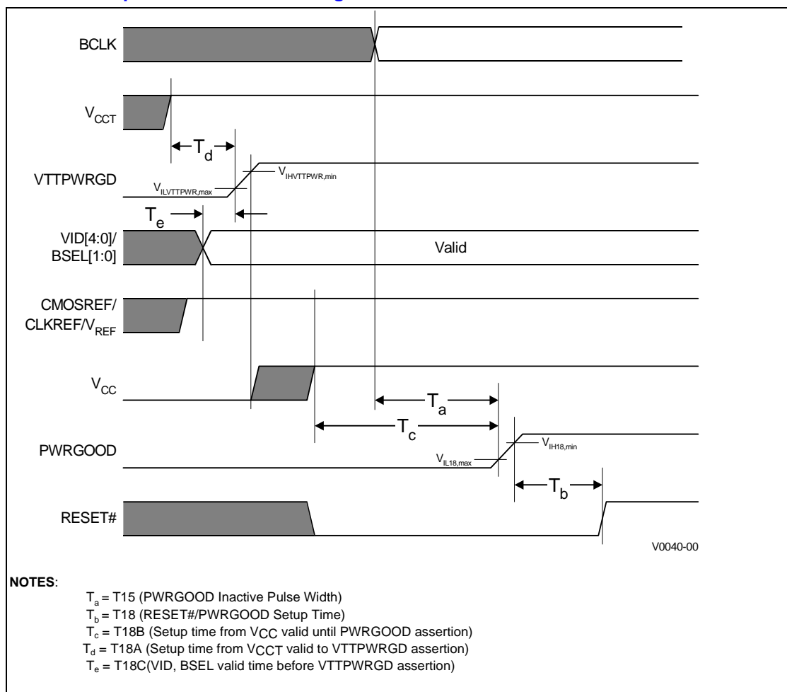
Figure 10. Power-on Sequence and Reset Timings
