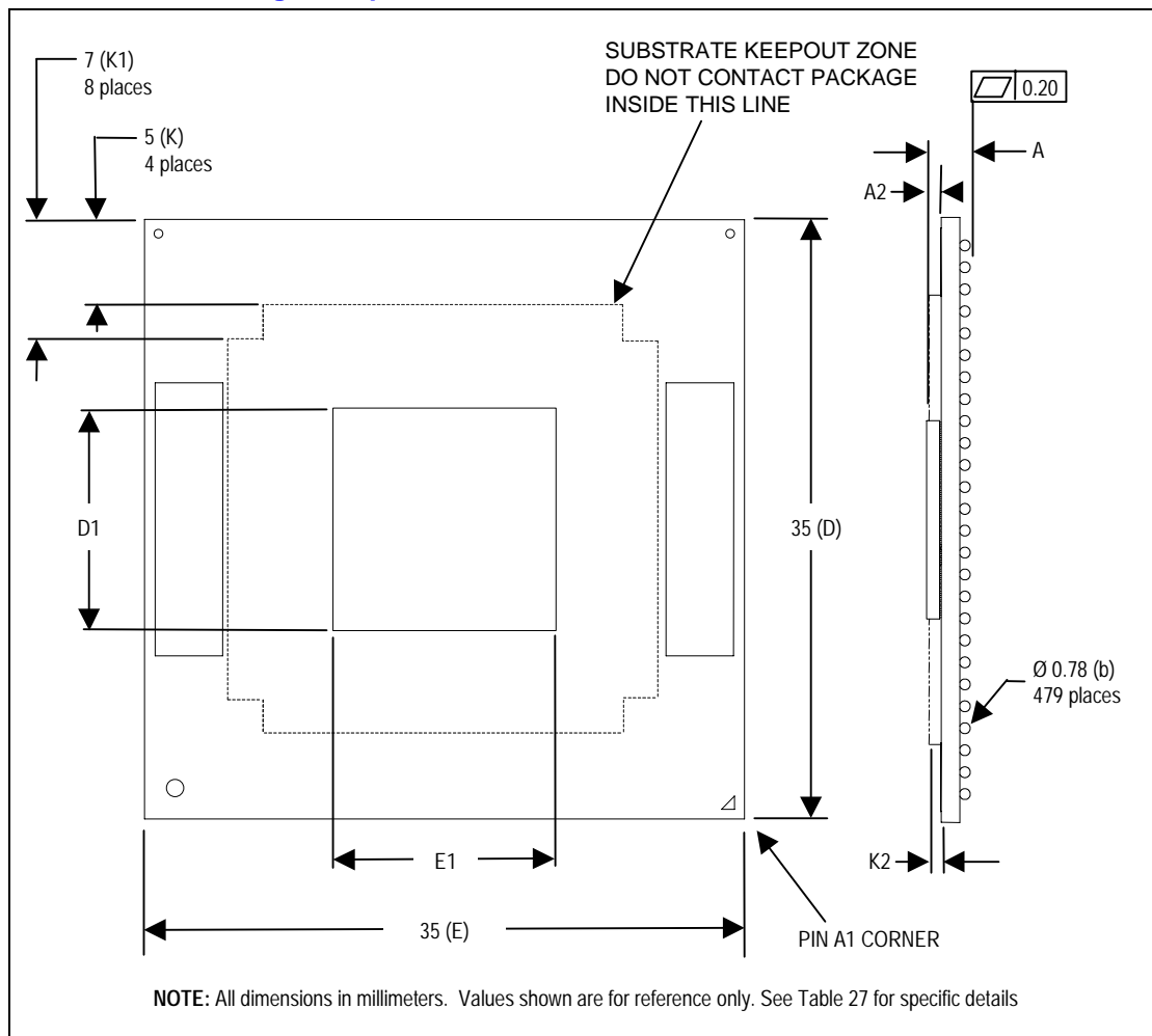
Figure 20. Micro-FCBGA Package – Top and Side Views
