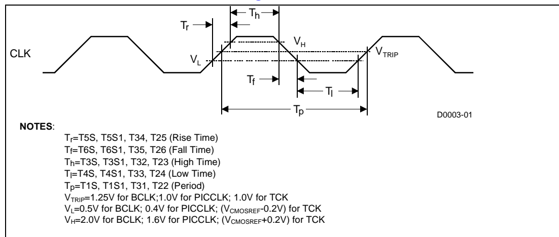
Figure 6. BCLK/PICCLK/TCK Generic Clock Timing Waveform
