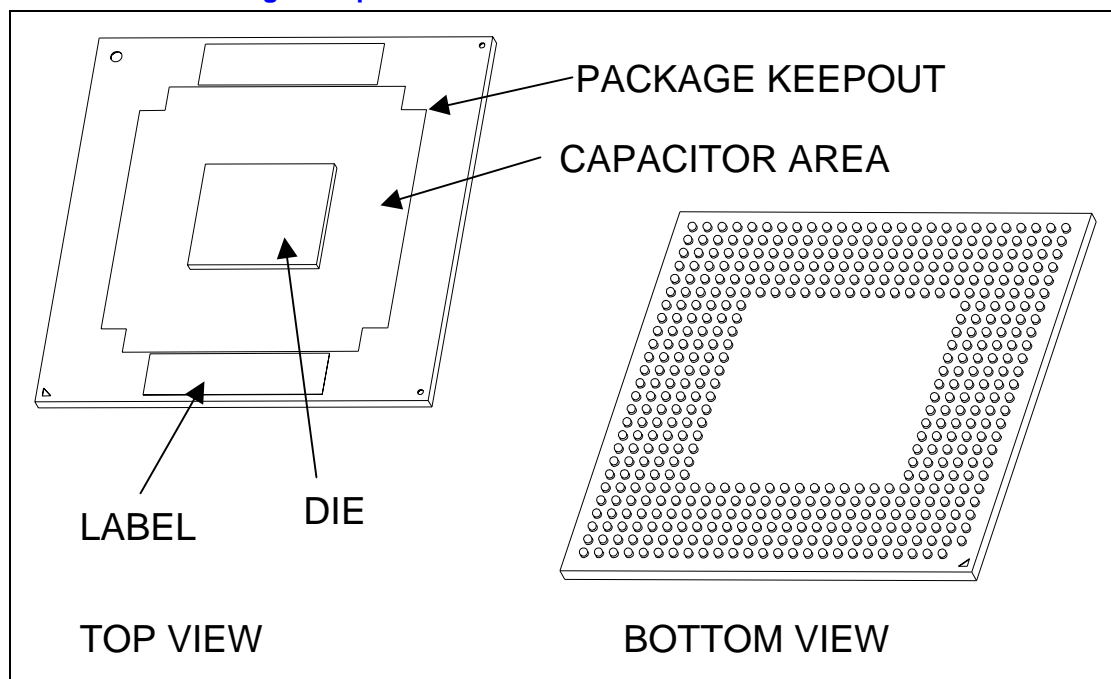
Figure 19. Micro-FCBGA Package – Top and Bottom Isometric Views
