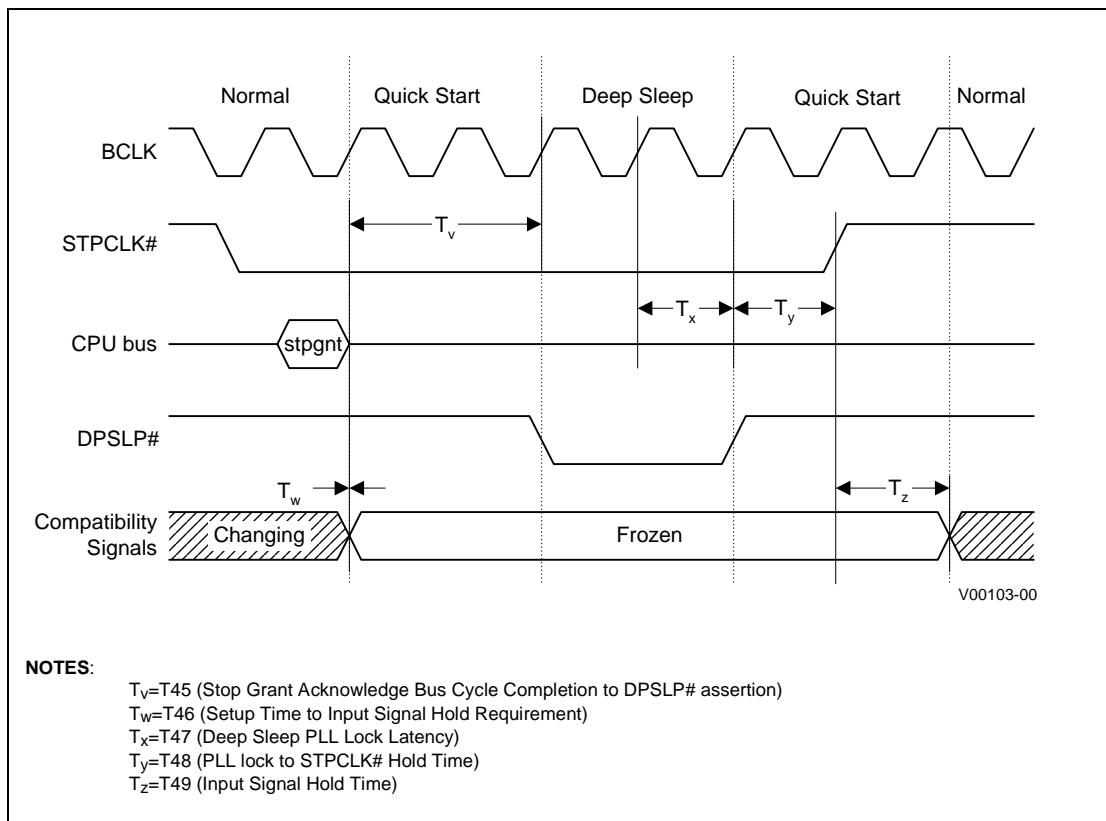
Figure 16. Quick Start/Deep Sleep Timing (DPSLP# Assertion Method)
