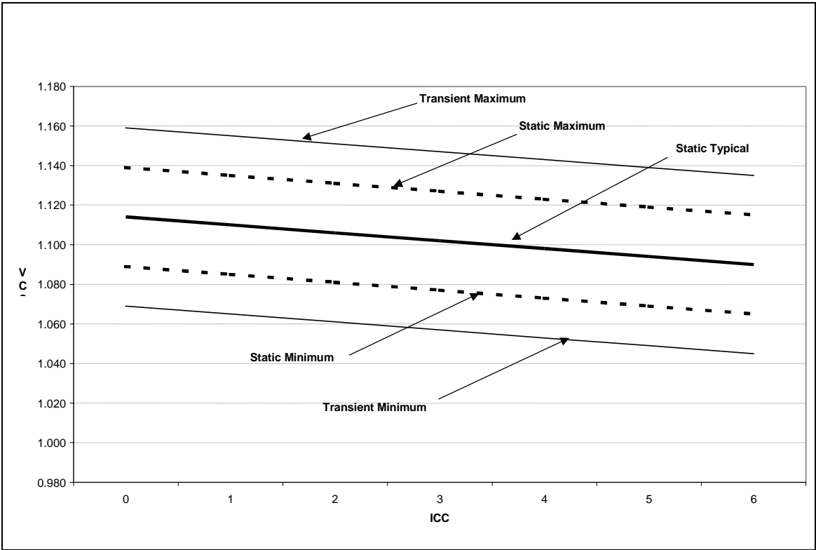
Figure 5. Illustration of Deep Sleep V_{CC} Static and Transient Tolerances (VID Setting = 1.15V)
