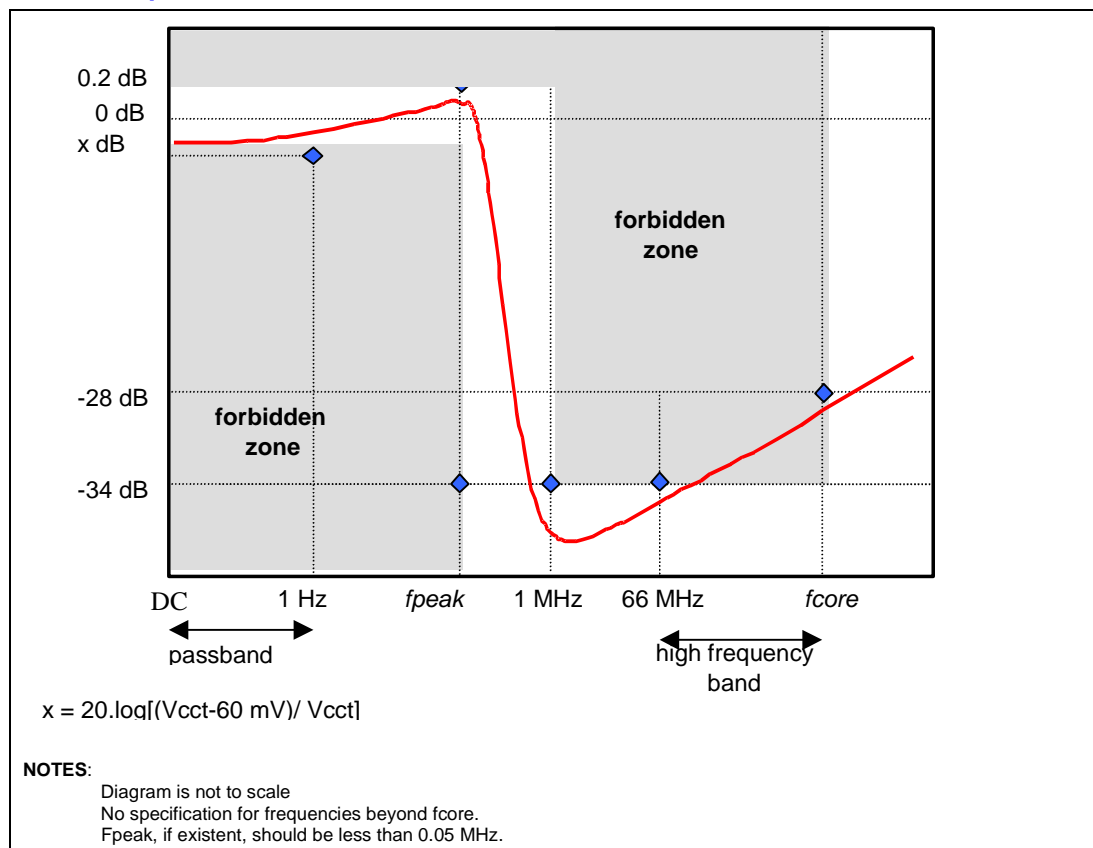
Figure 23. PLL Filter Specifications
