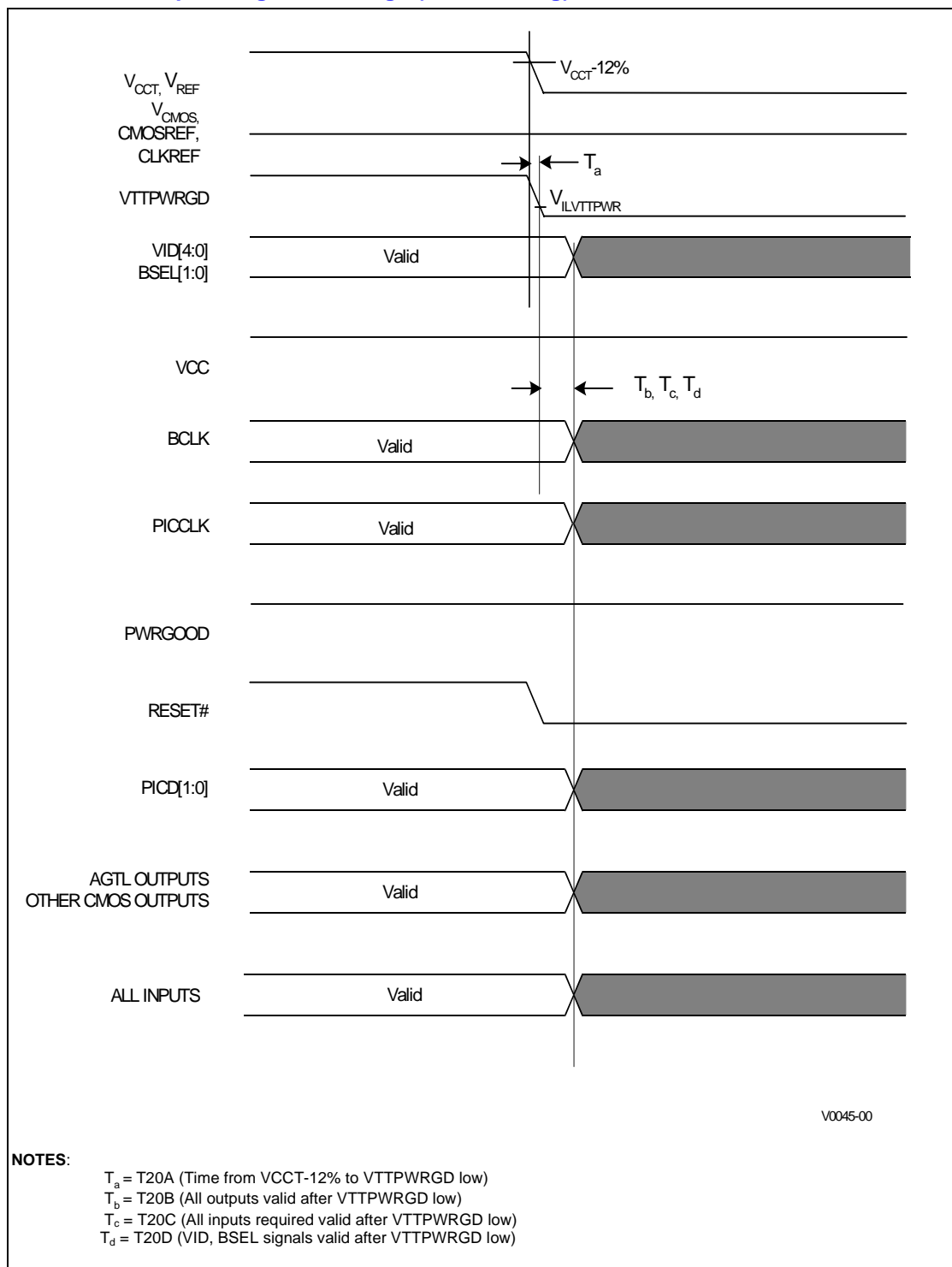
Figure 12. Power Down Sequencing and Timings (V CCT Leading)
