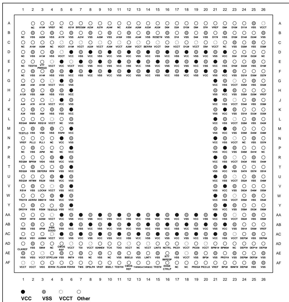
Figure 22. Pin/Ball Map - Top View
