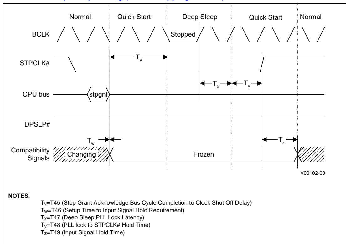
Figure 15.Quick Start/Deep Sleep Timing (BCLK Stopping Method)
