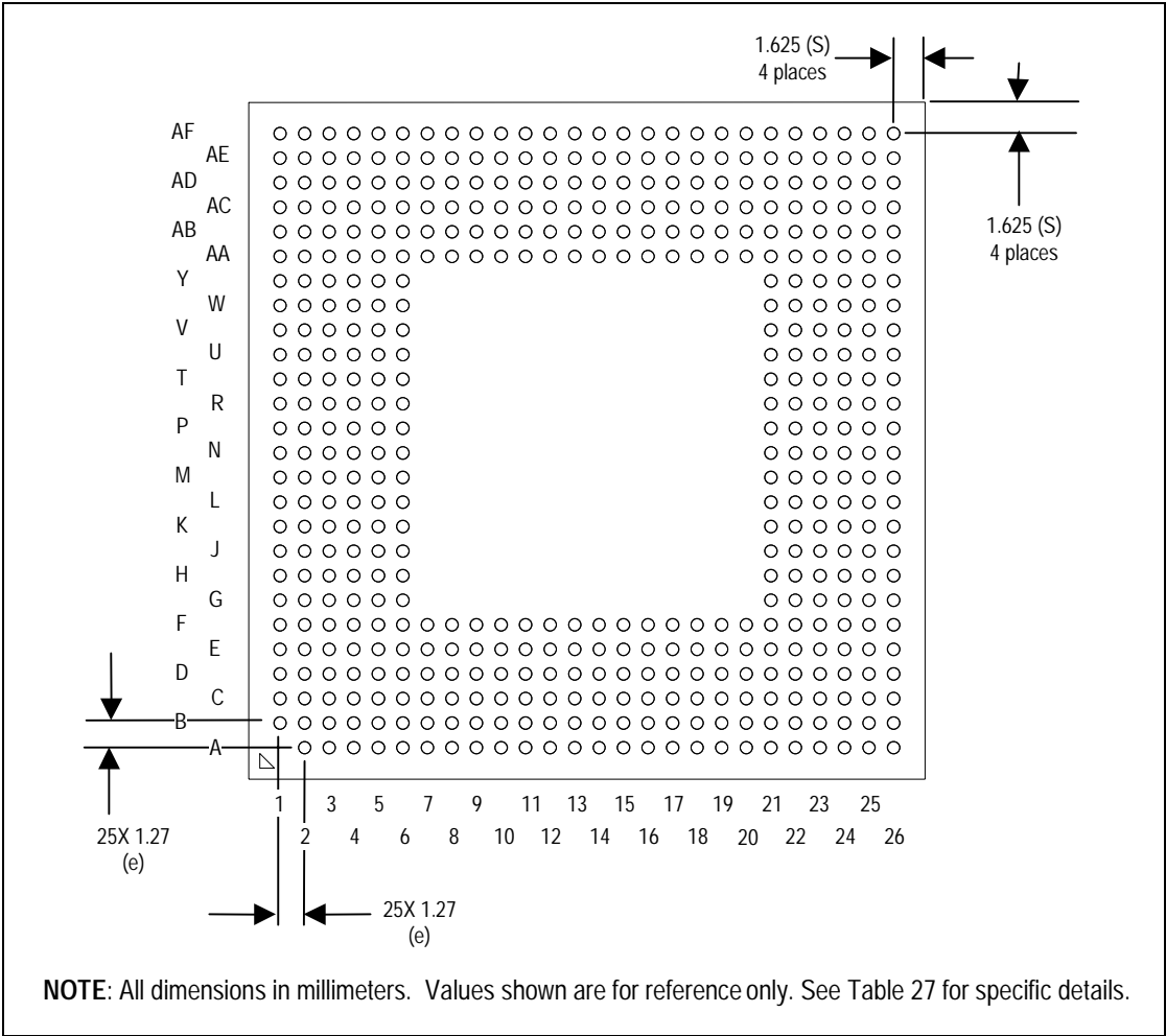
Figure 21. Micro-FCBGA Package - Bottom View
