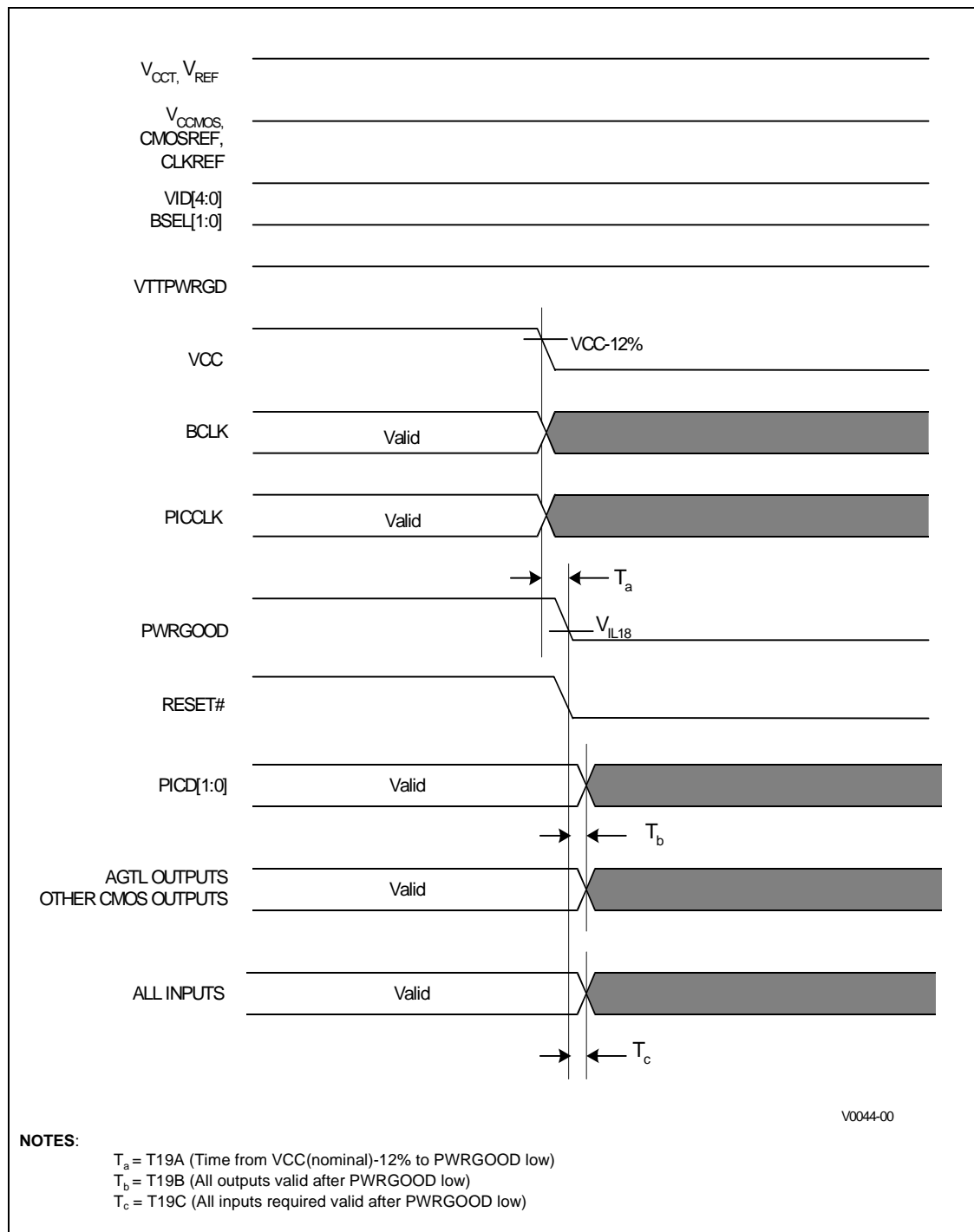
Figure 11. Power Down Sequencing and Timings (VCC Leading)
