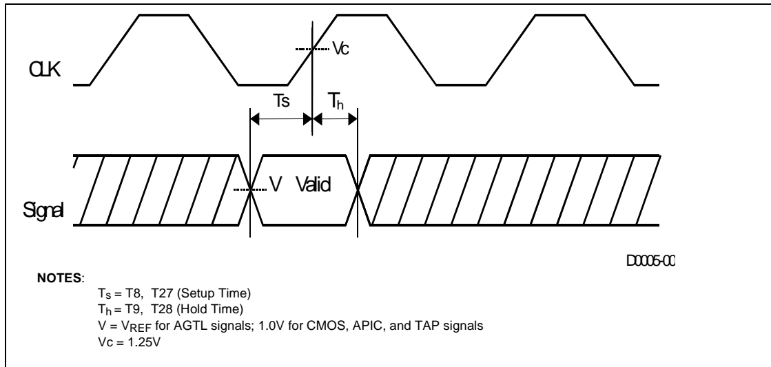
Figure 8. Setup and Hold Timings
