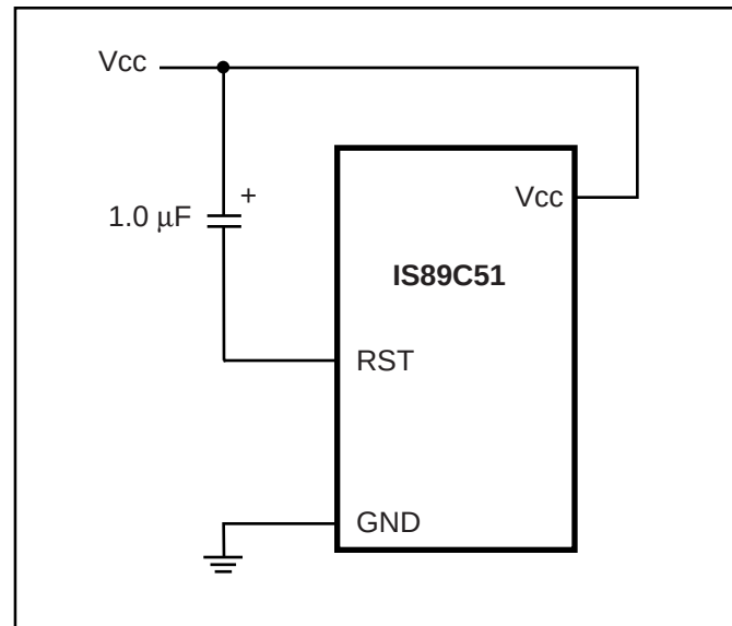
Figure 19. Power-On Reset Circuit
