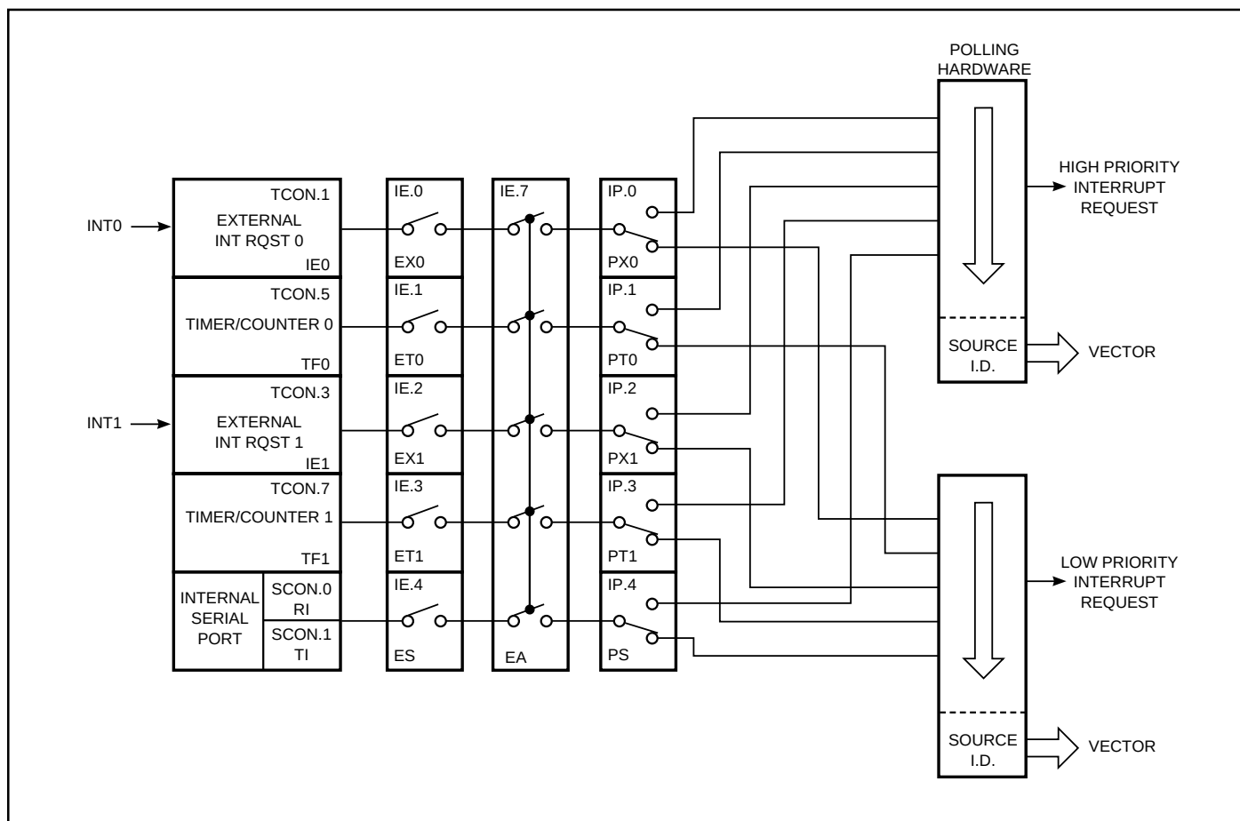
Figure 16. Interrupt System
