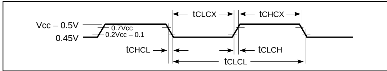
Figure 31. Icc Test Conditions
