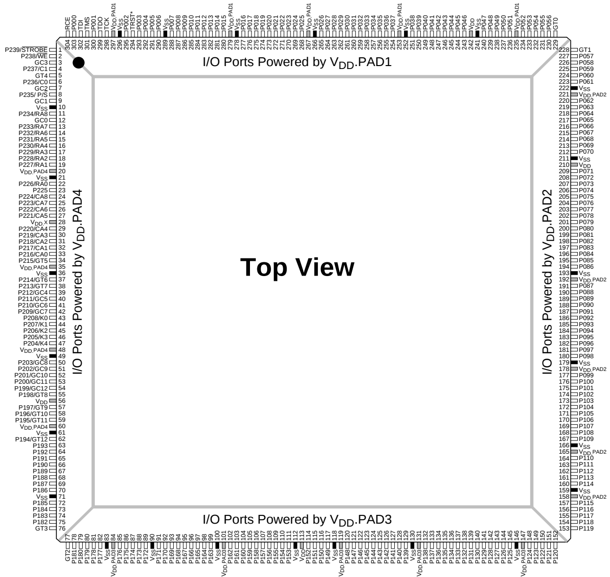
Figure 31. IQX240B [PQFP/304L] Package Pinout
