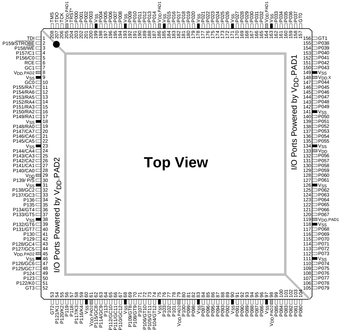
Figure 32. IQX160 [PQFP/208L] Package Pinout
