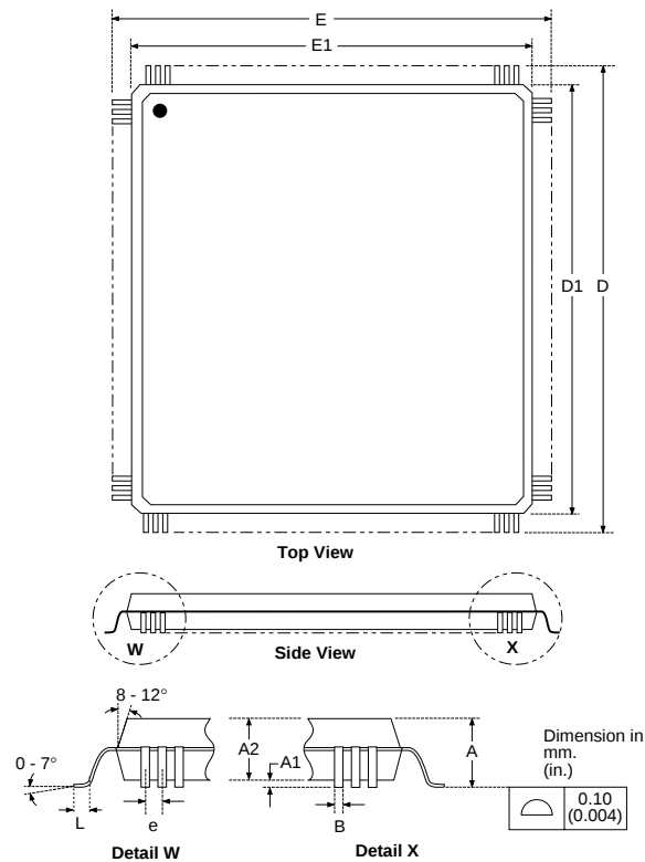
Figure 35. PQFP Package Dimensions
