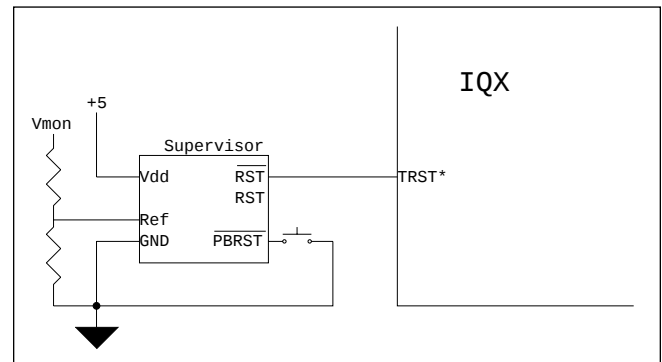
Figure 8. Reset Circuit
