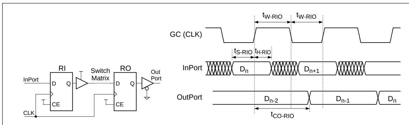
Figure 13. Registered Input and Registered Output Mode Timing (ICLK and OCLK are Synchronized)
