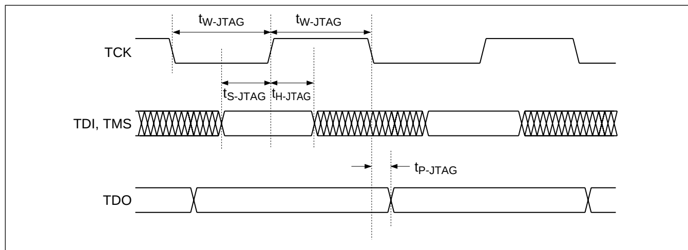
Figure 29. JTAG Timing
