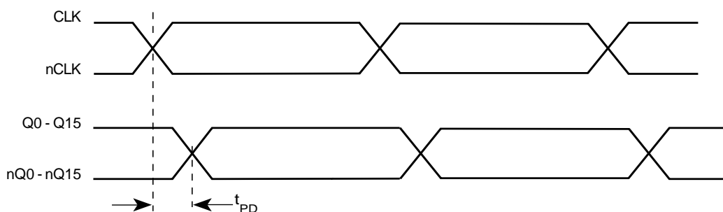
FIGURE 6 - PROPAGATION DELAY
