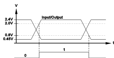
Fig. 2: reference levels
