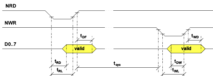
Fig. 3: read / write timing
