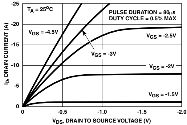
FIGURE 7. SATURATION CHARACTERISTICS
