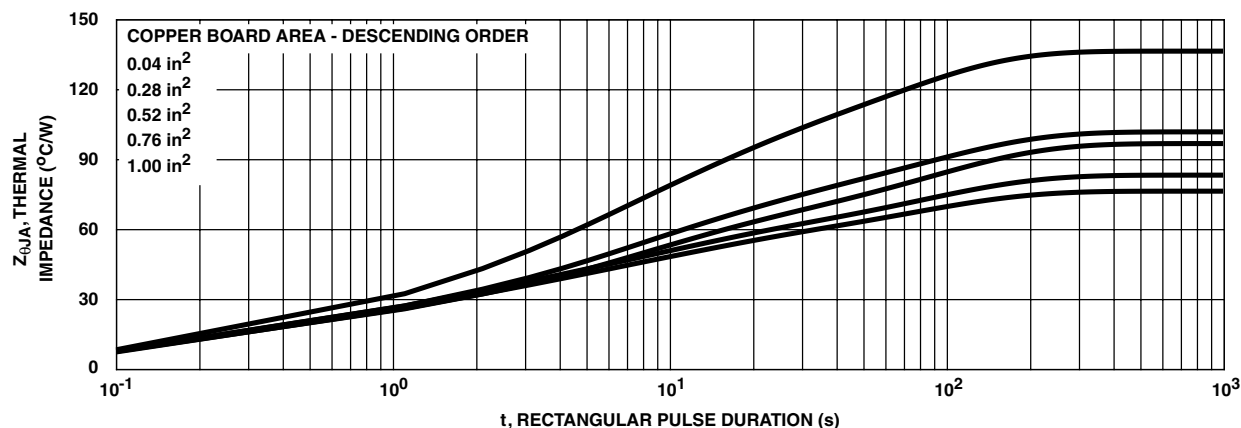
FIGURE 21. THERMAL IMPEDANCE vs MOUNTING PAD AREA
