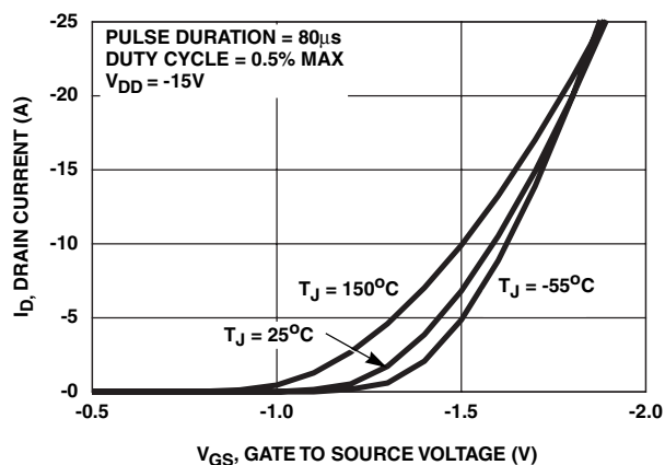
FIGURE 6. TRANSFER CHARACTERISTICS
