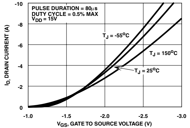
FIGURE 6. TRANSFER CHARACTERISTICS
