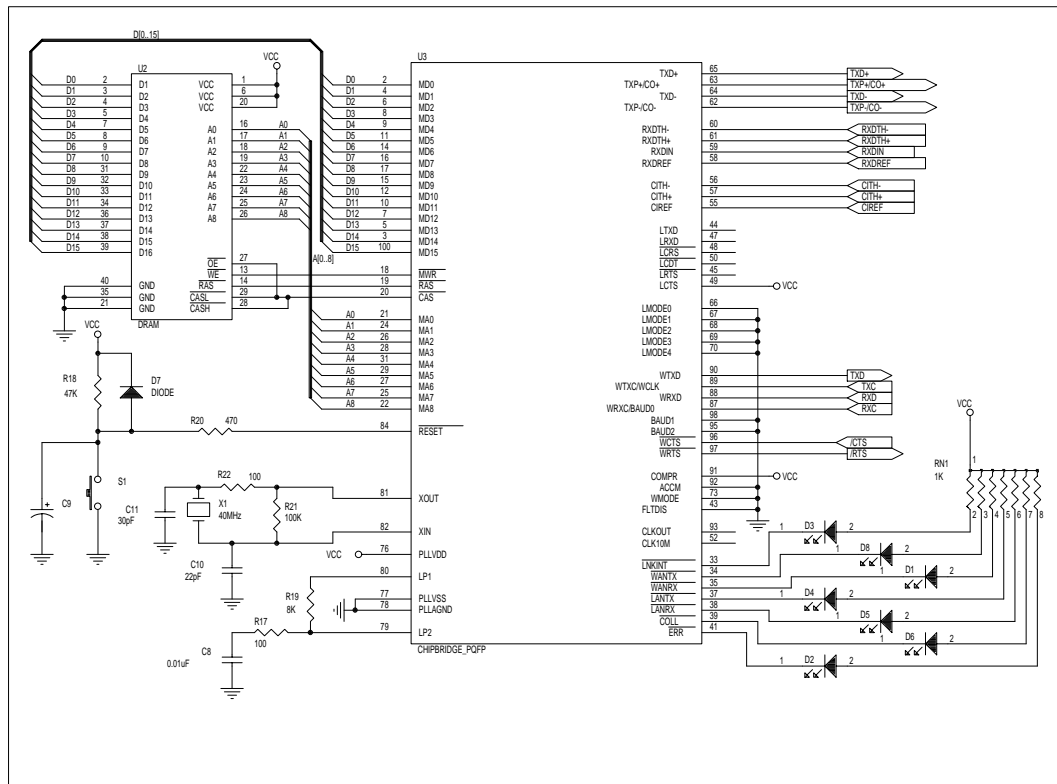
Figure 15. ChipBridge Connection
