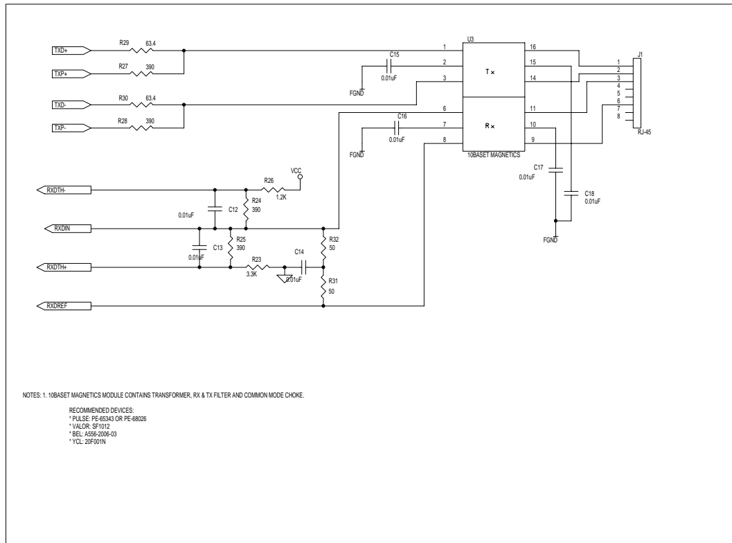
Figure 16. UTP Interface
