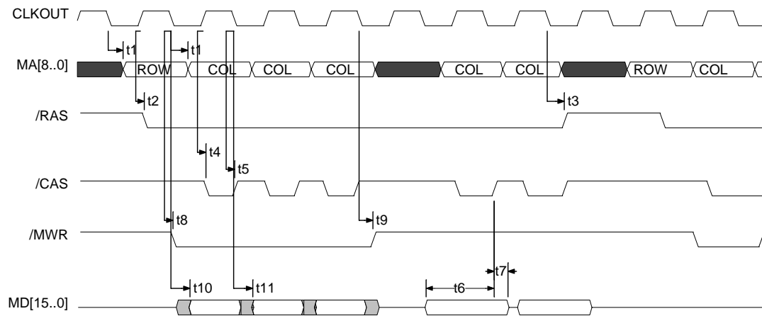
Figure 4. Burst-Mode DRAM Read and Write Timing
