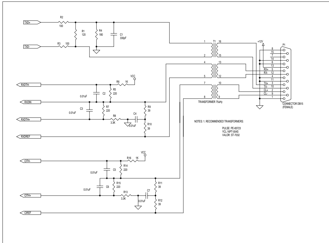
Figure 17. AUI-DTE Interface
