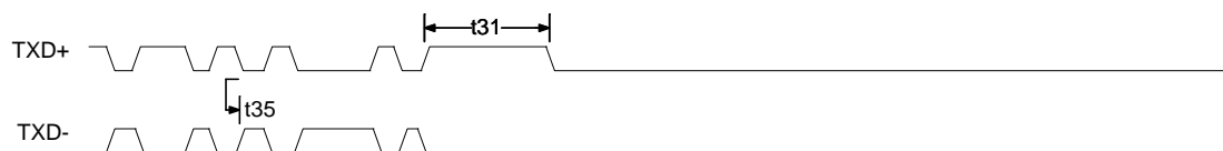
Figure 8. AUI-DTE Mode Timing
