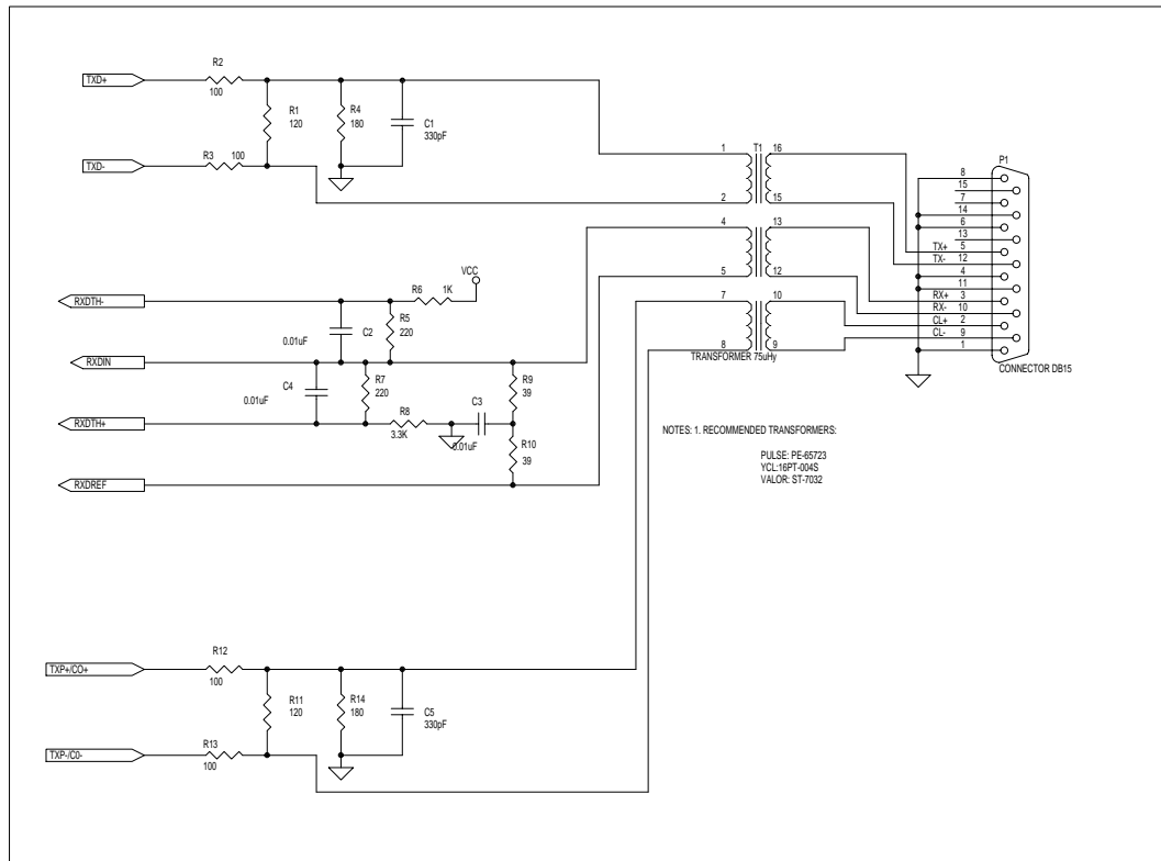
Figure 18. AUI-DCE Interface
