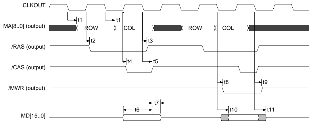
Figure 3. Single Cycle DRAM Read and Write Timing
