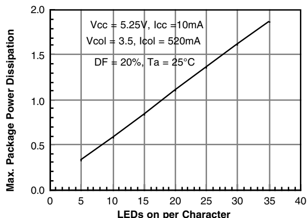
Figure 14. Max. Package Power Dissipation, ISD235X
