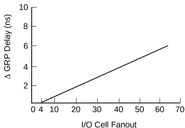
Maximum \Delta GRP Delay vs. I/O Cell Fanout
