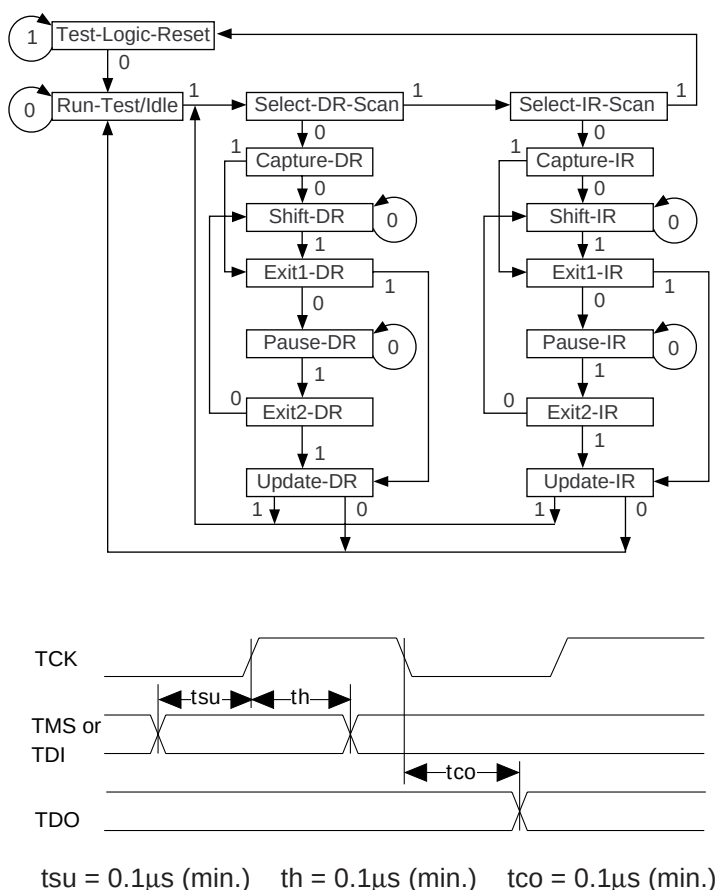
Figure 8. Boundary Scan State Machine
