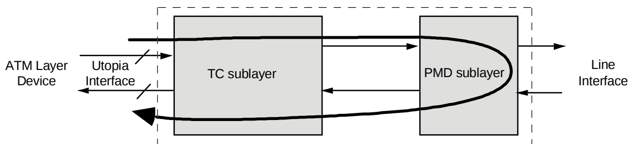
Figure 13. PHY Loopback
