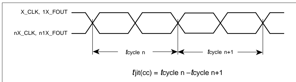
FIGURE 2 — CYCLE-TO-CYCLE JITTER
