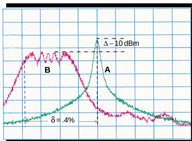
FIGURE 3. 200MHz CLOCK OUTPUT IN FREQUENCY DOMAIN
