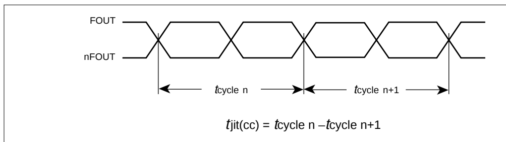
FIGURE 2 — CYCLE-TO-CYCLE JITTER
