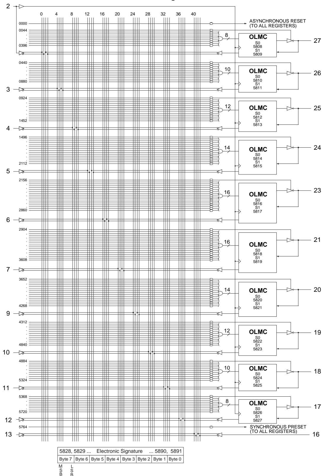
PLCC & SSOP Package Pinout
