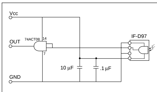
FIGURE 3. Typical interface circuit.
