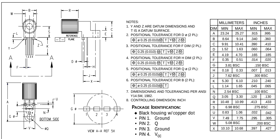
FIGURE 4. Case outline.
