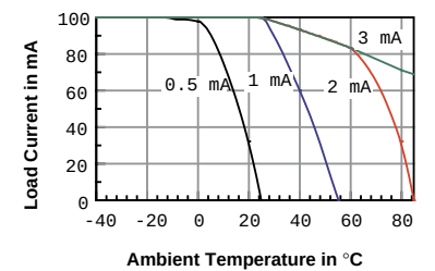
Figure 3. SSR turn-on current versus temperature
