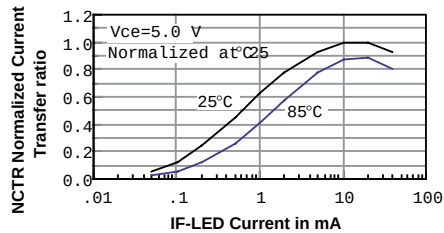
Figure 10. Non-saturated current transfer ratio, typical
