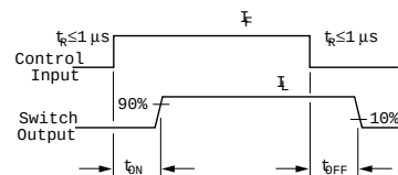
Figure 12. Switching waveform
