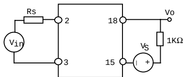
Figure 11. Switching test circuit for SSR channel
