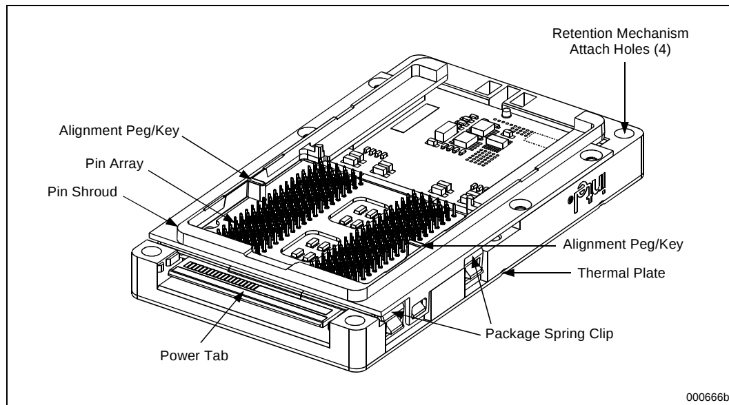
Figure 4-2. Intel® Itanium™ Processor PAC418 Bottom Isometric View
