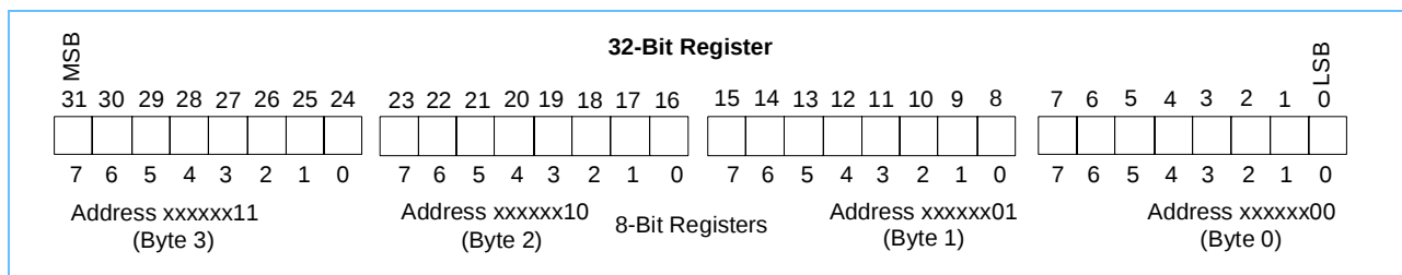
Figure 28: Register Addressing
