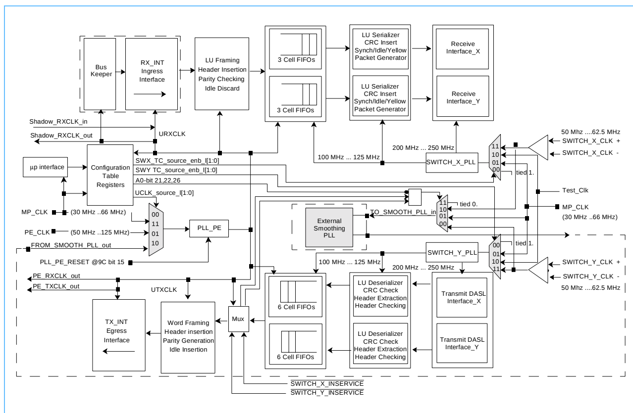
Figure 21: Clocks Distribution Diagram
