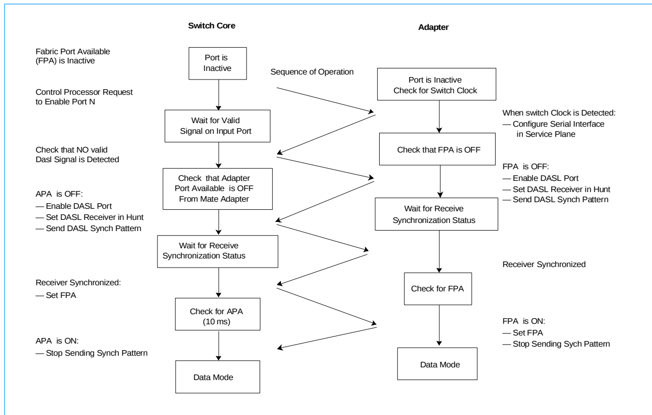
Figure 41: Switch Fabric DASL Port Synchronization Sequence
