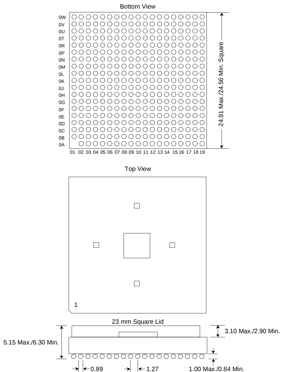
Figure 39: CBGA 25 mm x 25 mm 360-Lead Schematic
