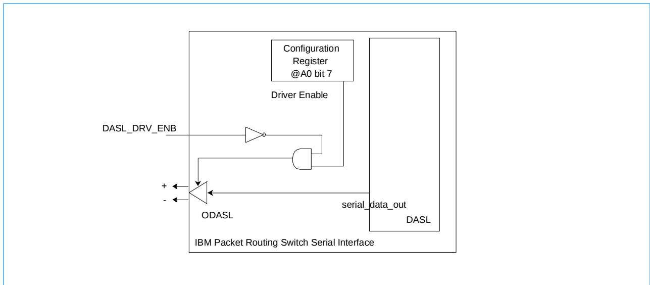
Figure 32: Enabling of Data Aligned Serial Link (DASL) Data Transmission and Reception Path Y
