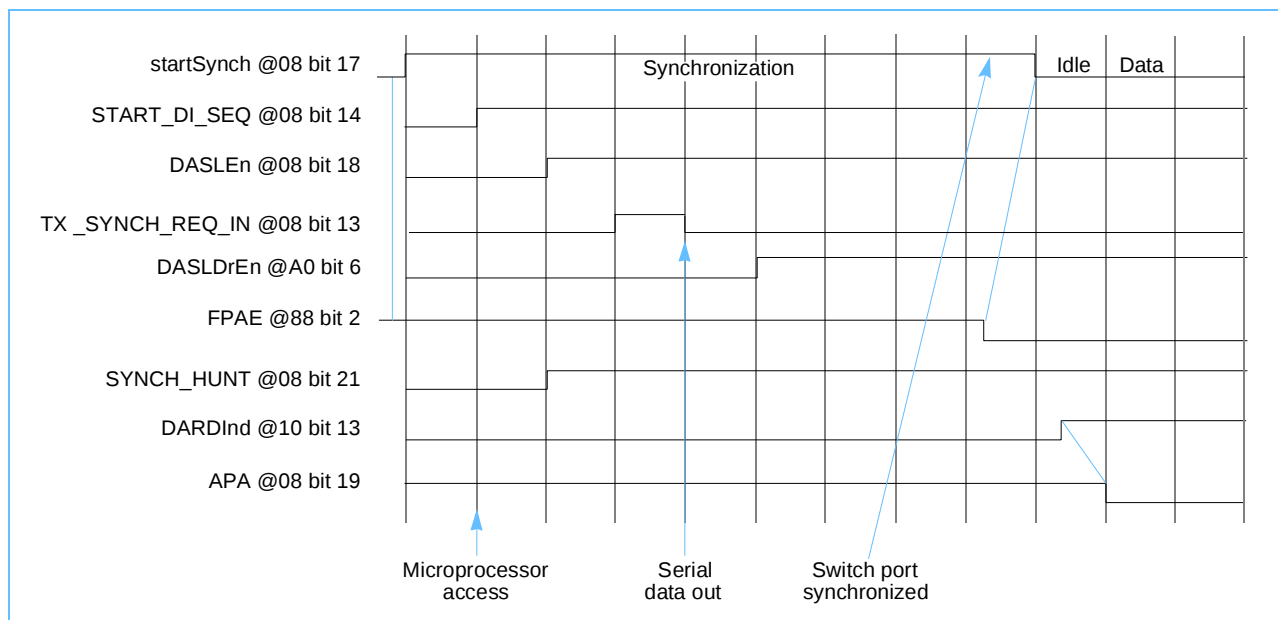
Figure 30: Enabling of Data Aligned Serial Link (DASL) Data Transmission and Reception Path X
