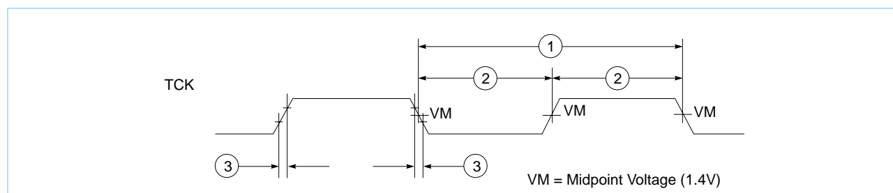
Figure 16. JTAG Clock Input Timing Diagram
