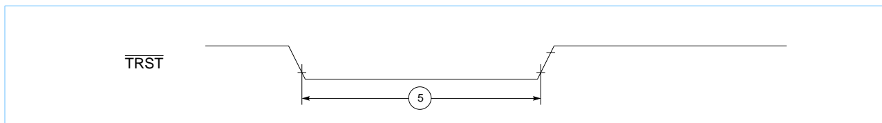
Figure 17. \overline{\text{TRST}} Timing Diagram
