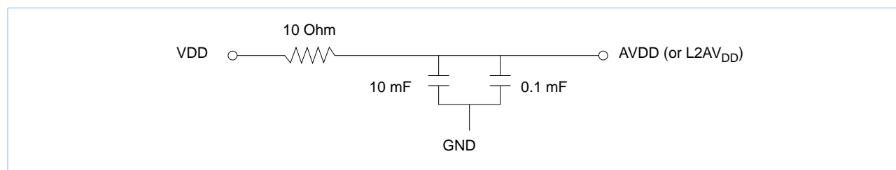
Figure 22. PLL Power Supply Filter Circuit
