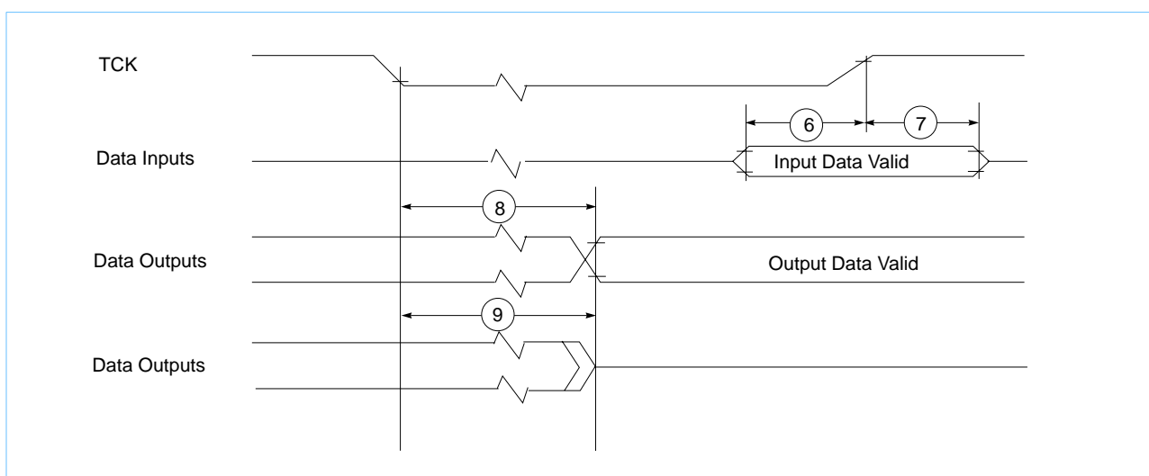
Figure 18. . Boundary-Scan Timing Diagram
