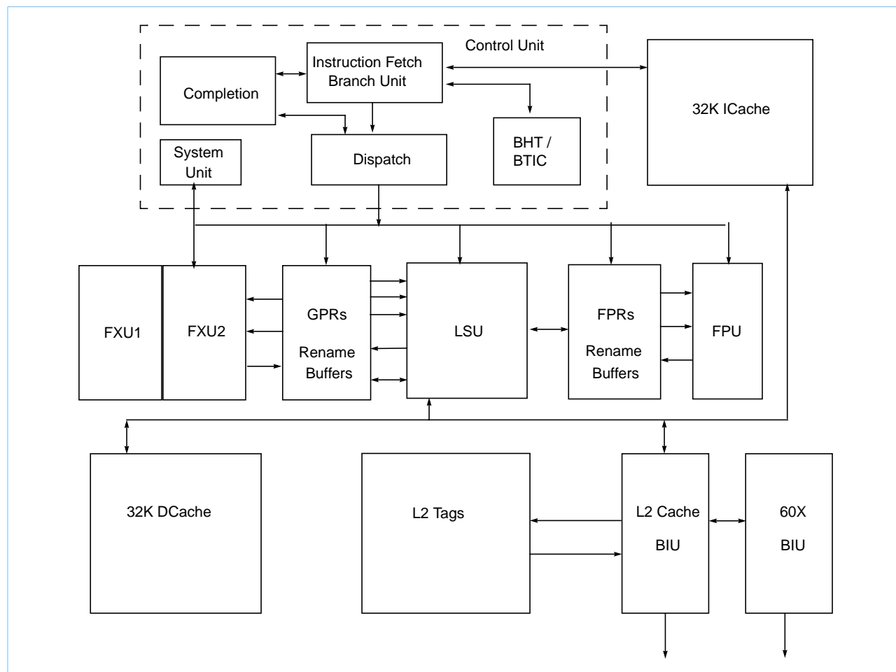
Figure 8. 750 Block Diagram.
