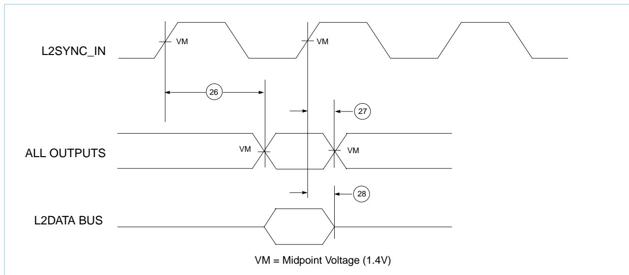
Figure 15. L2 Bus Output Timing Diagrams
