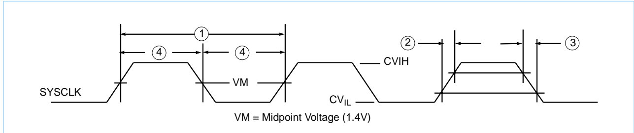
Figure 9. SYCLK Input Timing Diagram
