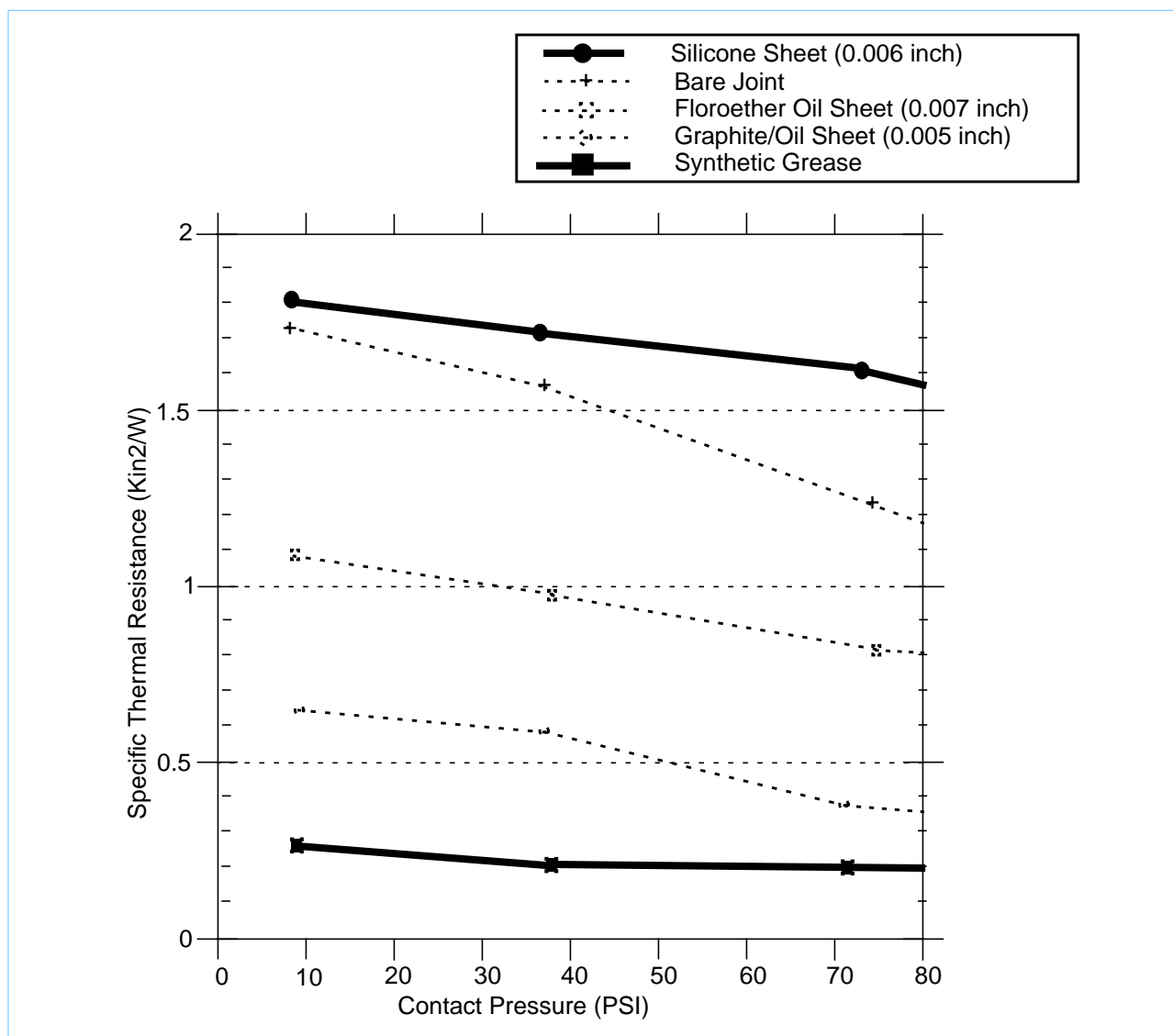
Figure 26. Thermal Performance of Select Thermal Interface Material
