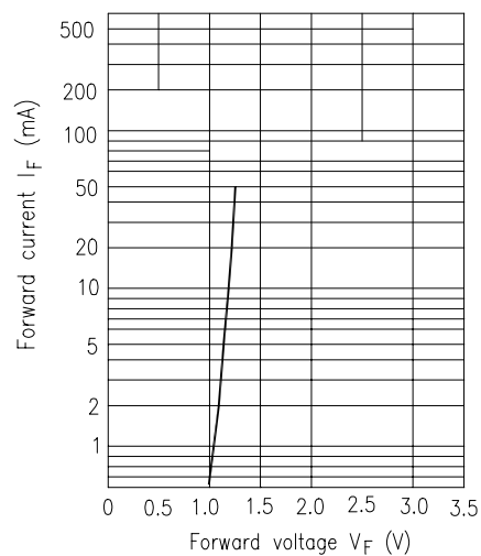
Fig. 4 Forward Current vs. Forward Voltage
