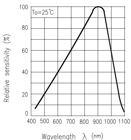
Fig.3 Spectral Sensitivity
