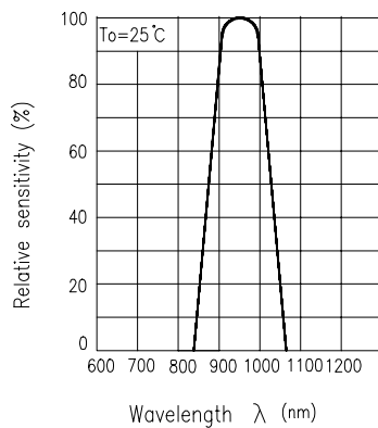
Fig.5 Spectral Sensitivity
