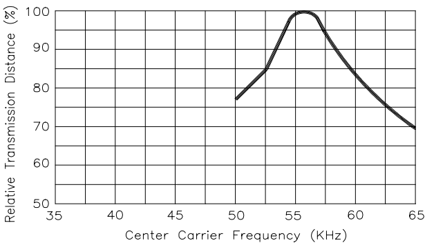
Fig.-8 Relative Transmission Distance vs. Center Carrier Frequency
