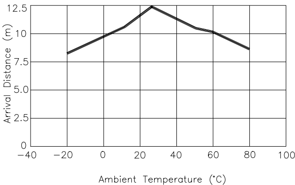
Fig.-9 Arrival Distance vs. Ambient Temperature
