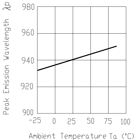
Fig. 3 Peak Emission Wavelength \lambda_p vs. Ambient Temperature
