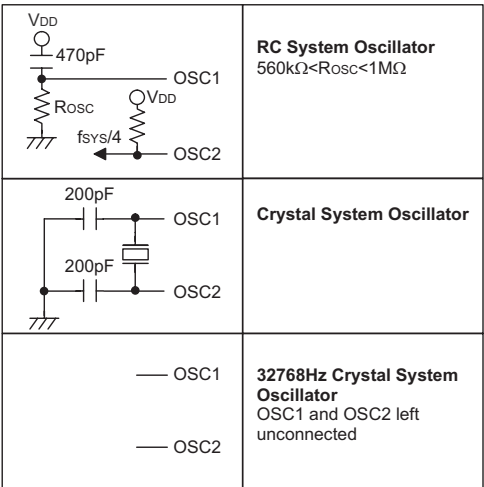
OSC Circuit
