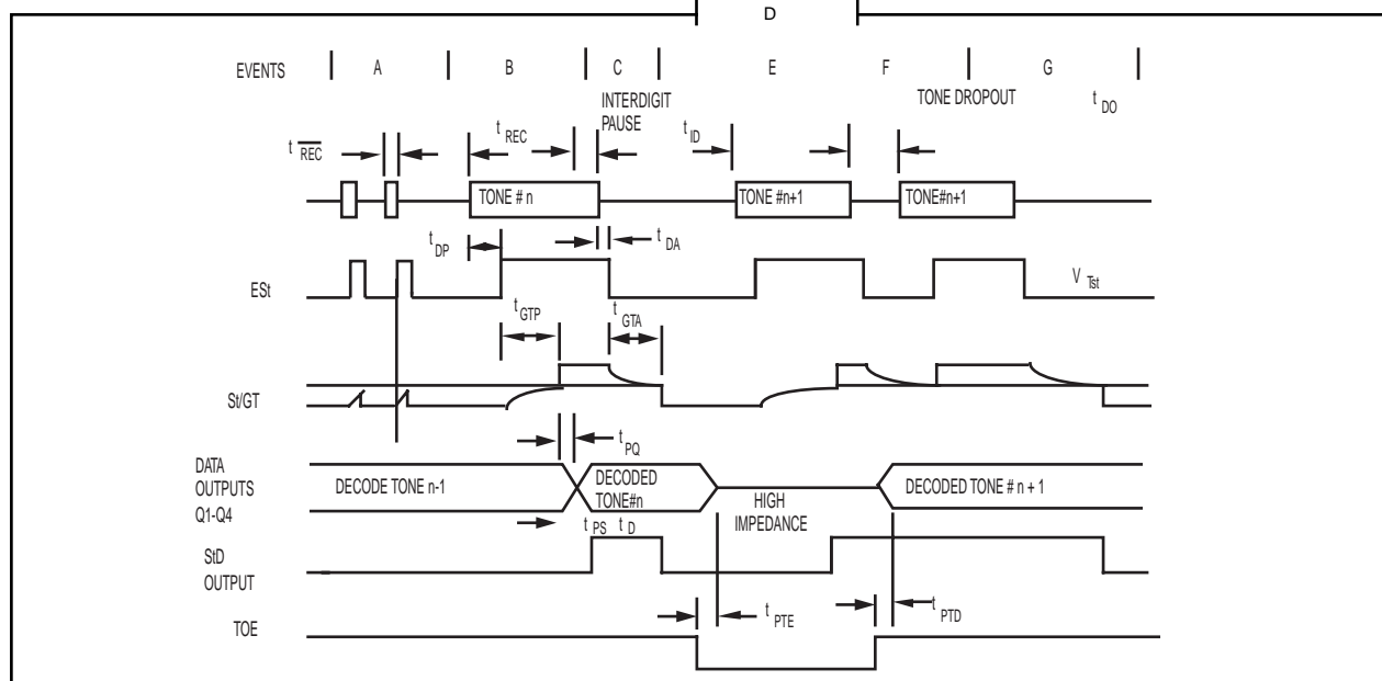
FIGURE 5. TIMING DIAGRAM
