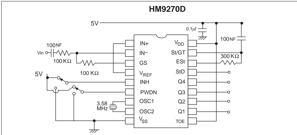
FIGURE 3. SINGLE ENDED INPUT CONFIGURATION
