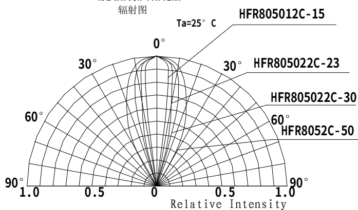
RADIATION PATTERN
