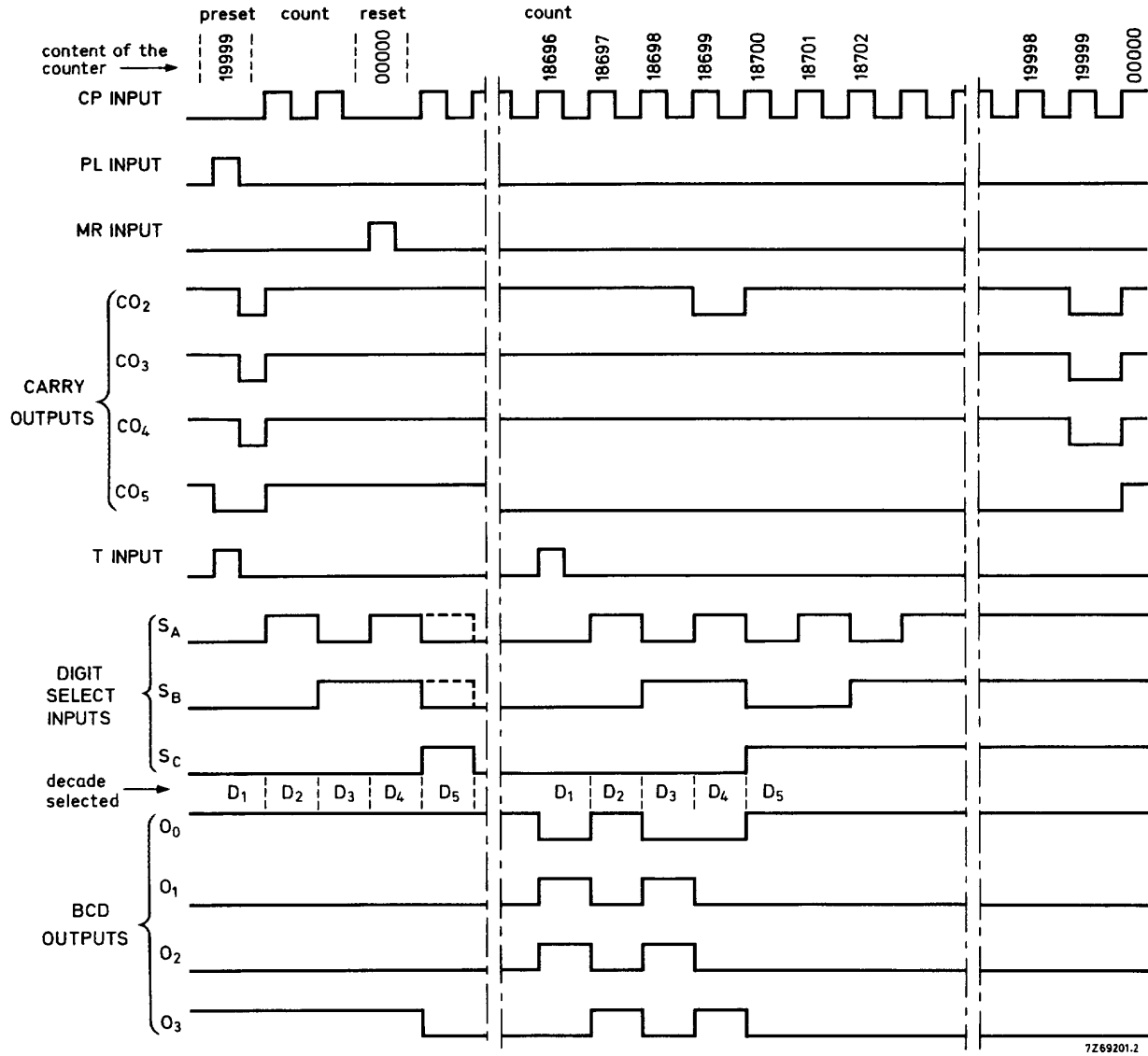
Fig.3 Timing diagram.
