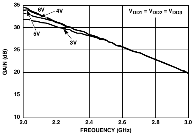
FIGURE 1. LINEAR GAIN
