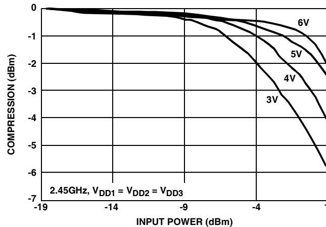
FIGURE 6. GAIN COMPRESSION
