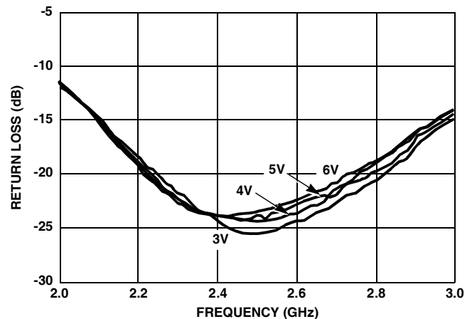
FIGURE 2. INPUT MATCH
