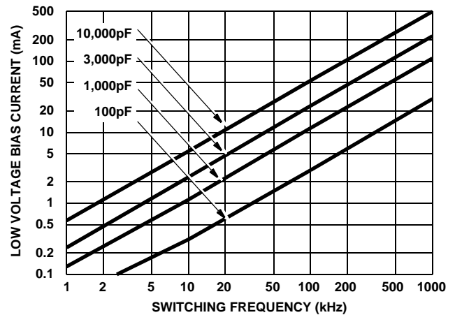
FIGURE 27. LOW VOLTAGE BIAS CURRENT I_{DD} (LESS QUIESCIENT COMPONENT) vs FREQUENCY AND GATE LOAD CAPACITANCE
