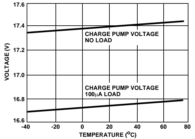
FIGURE 8. PUMP VOLTAGE
