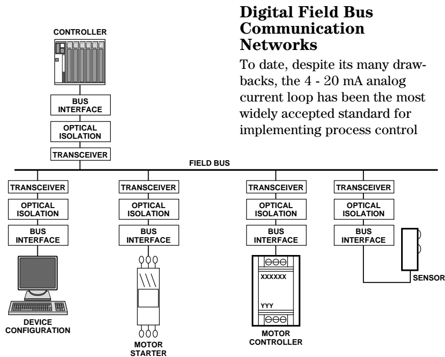
Figure 15. Typical Field Bus Communication Physical Model.
