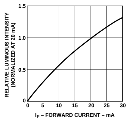
Figure 5. Blue, green relative luminous intensity vs. forward current.
