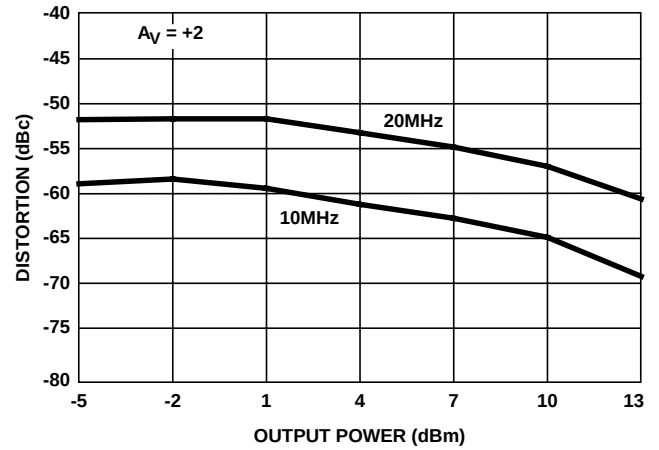
FIGURE 23. 3rd HARMONIC DISTORTION vs P_{\text{OUT}}
