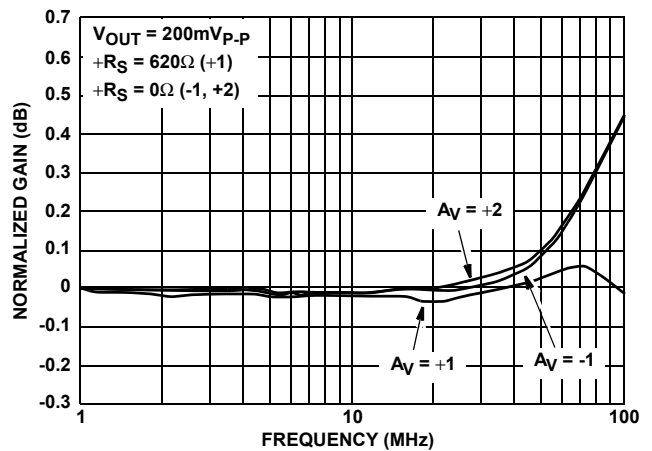
FIGURE 15. GAIN FLATNESS
