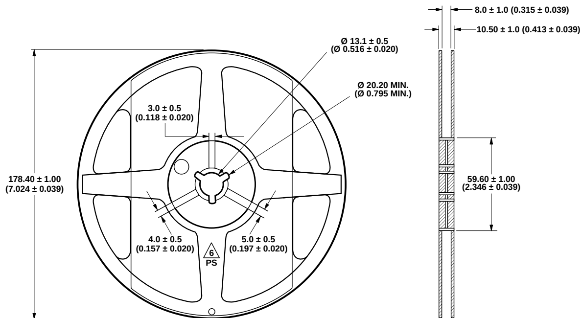
Figure 18. Reel Dimensions.
