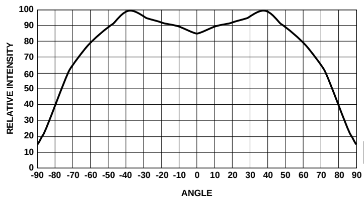
Figure 6. Relative Intensity vs. Angle for HSMx-C120.
