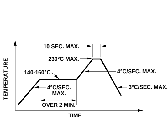
Figure 9. Recommended Reflow Soldering Profile.
