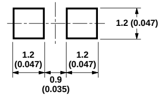
Figure 8. Recommended Soldering Pattern for HSMB-C170.
