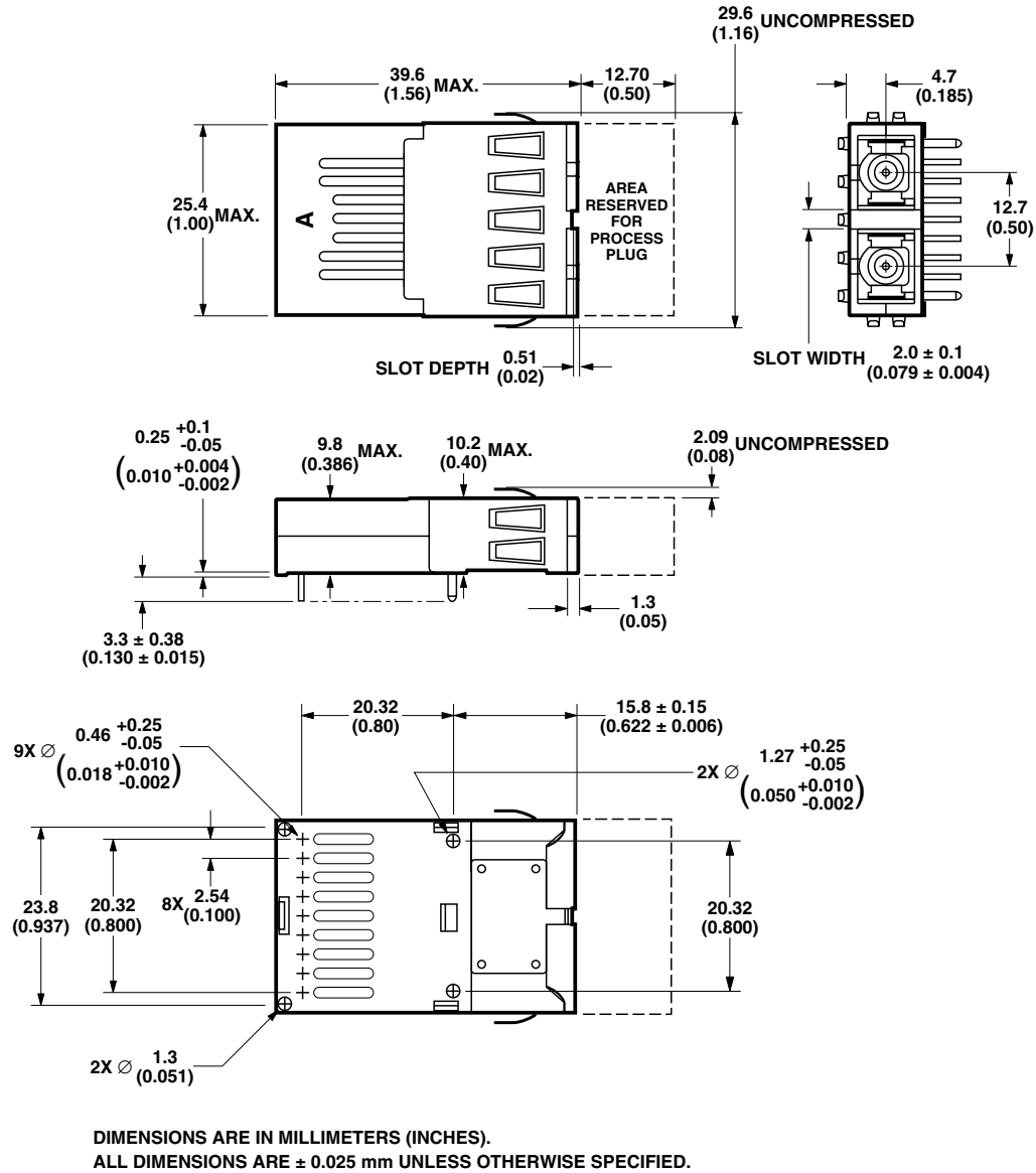
Figure 2b. Package Outline Drawing – Mezzanine Height with Extended Shield.
