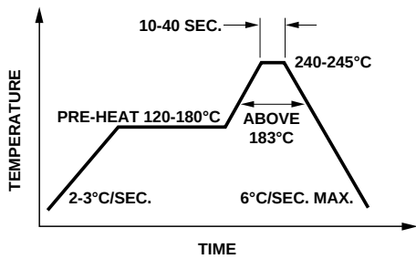
Figure 8a. Recommended wave soldering profile.
