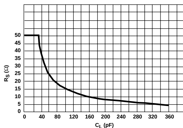
FIGURE 14. RECOMMENDED SERIES OUTPUT RESISTOR vs C_{\text{LOAD}}
