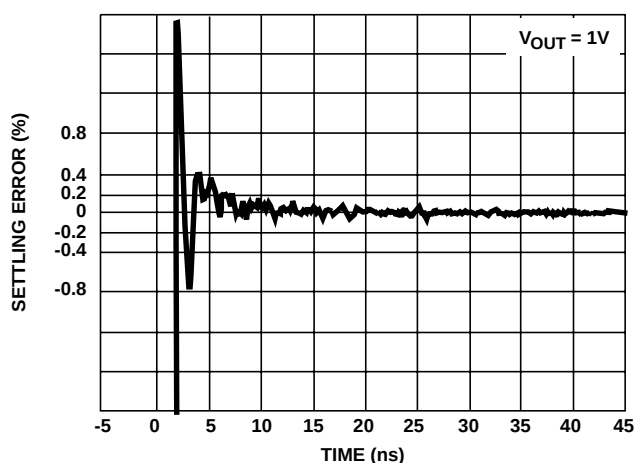
FIGURE 13. SETTLING RESPONSE
