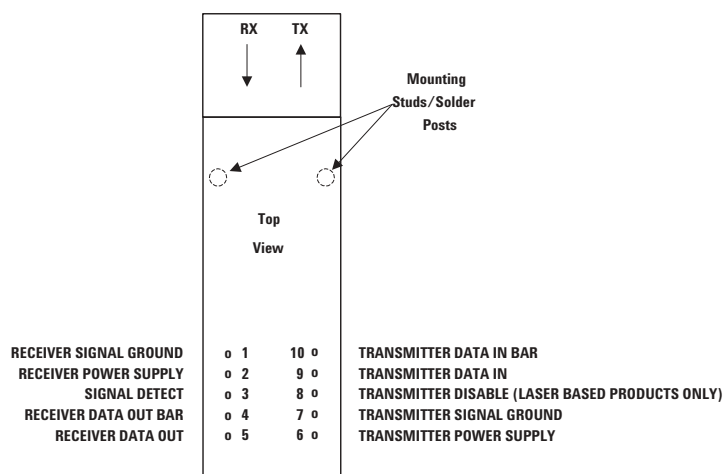
Figure 2. Pin Out Diagram
