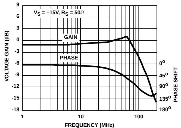
FIGURE 5. GAIN/PHASE vs FREQUENCY (R L = 50Ω)
