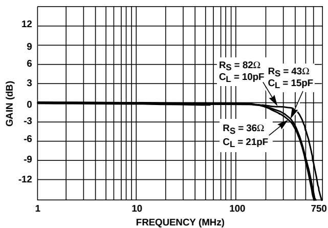
FIGURE 5. FREQUENCY RESPONSE
