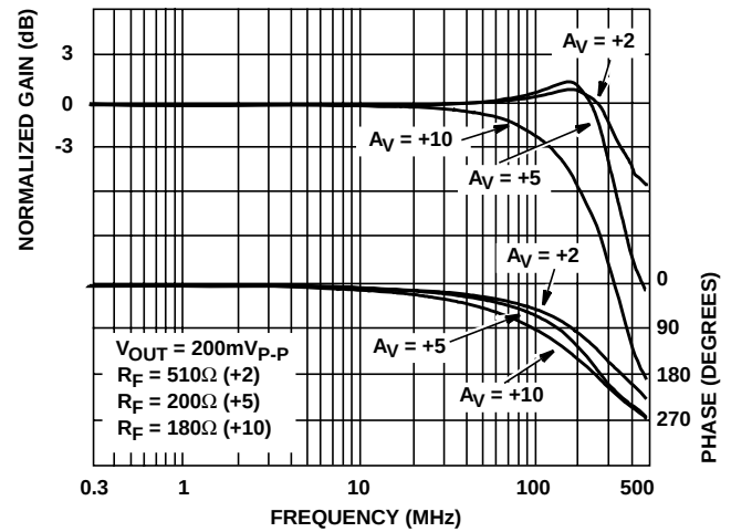
FIGURE 14. FREQUENCY RESPONSE
