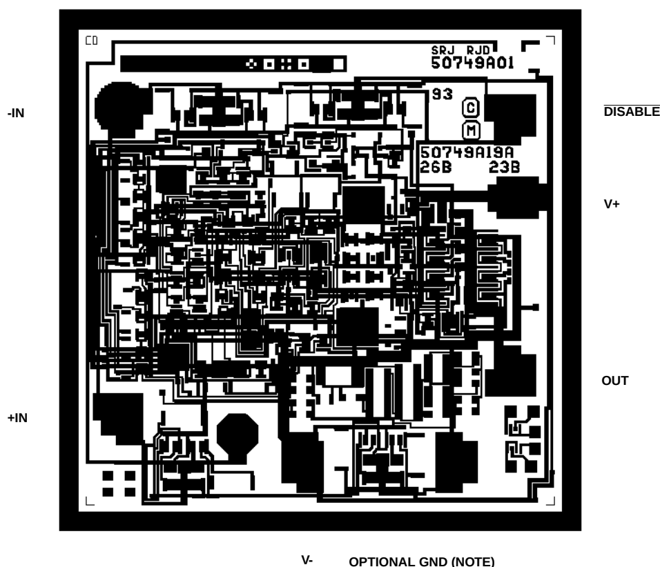
HFA1145
