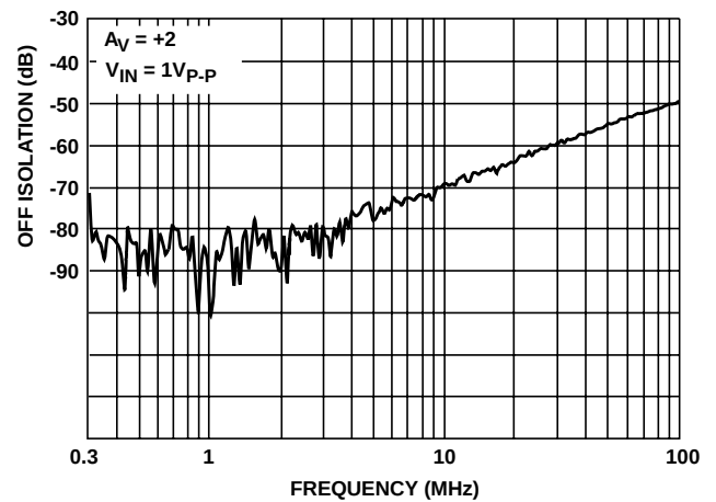
FIGURE 20. OFF ISOLATION
