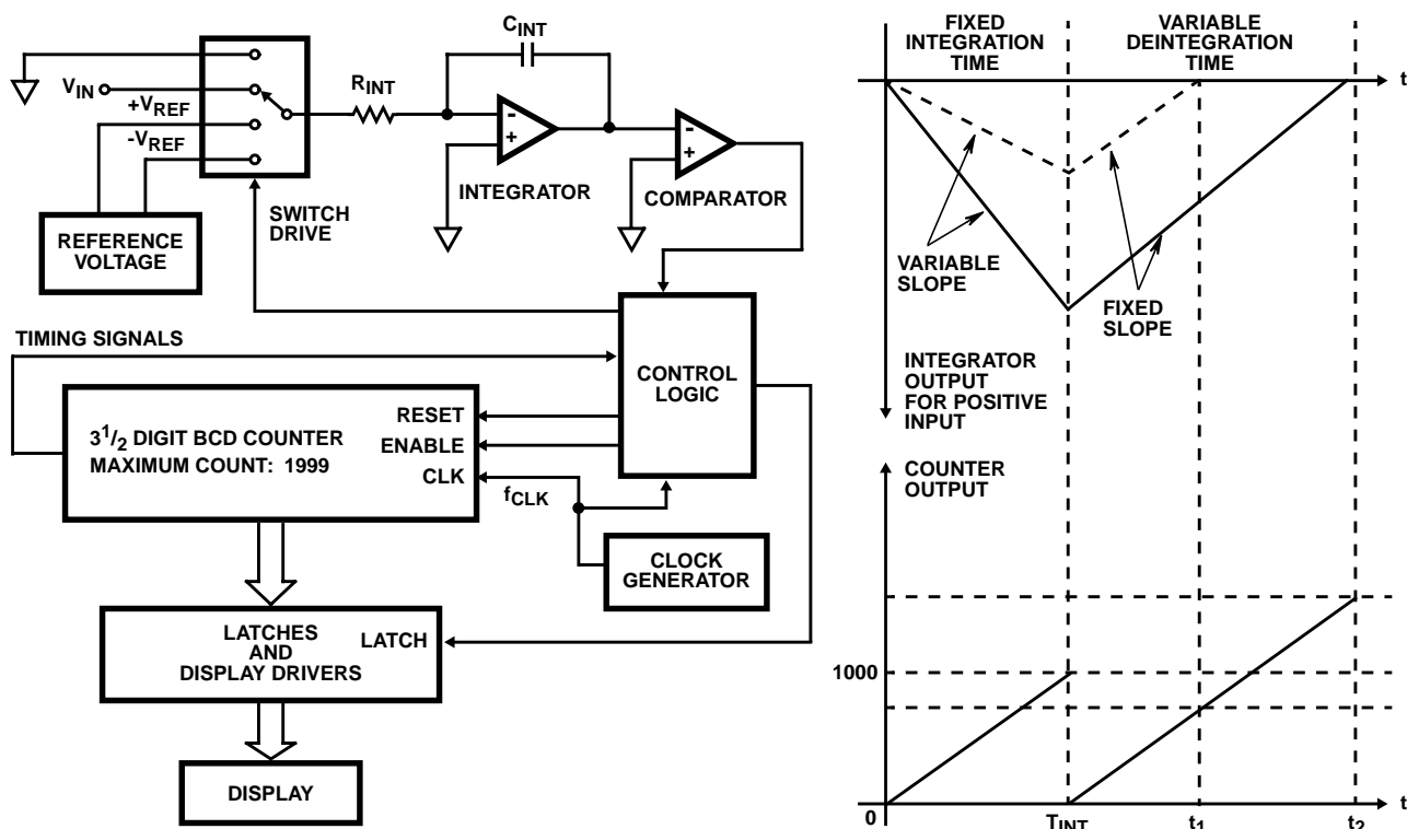
FIGURE 91. DUAL SLOPE INTEGRATING A/D CONVERTER
