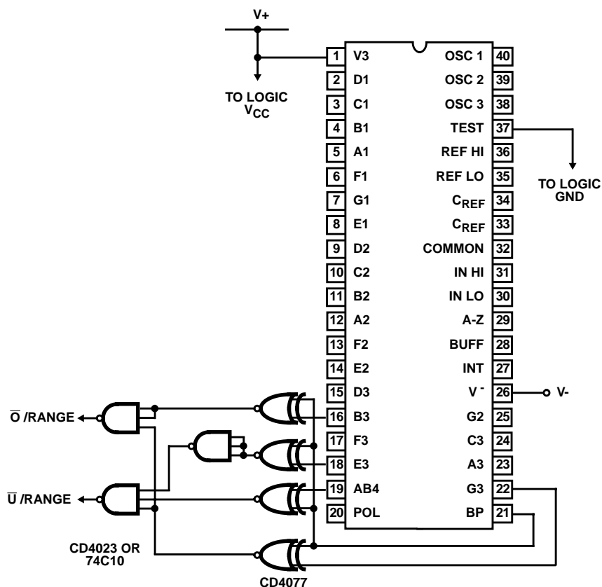
FIGURE 107. CIRCUIT FOR DEVELOPING UNDERRANGE AND OVERRANGE SIGNALS FROM HI7131 OUTPUTS
