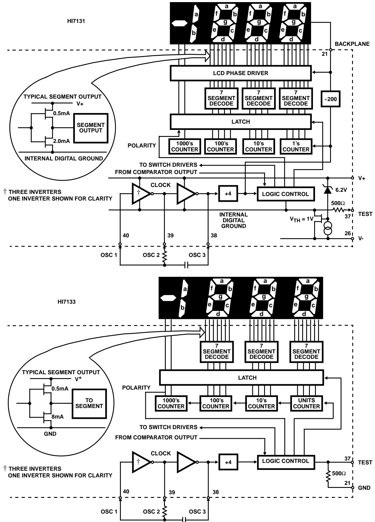
FIGURE 94. DIGITAL SECTION
